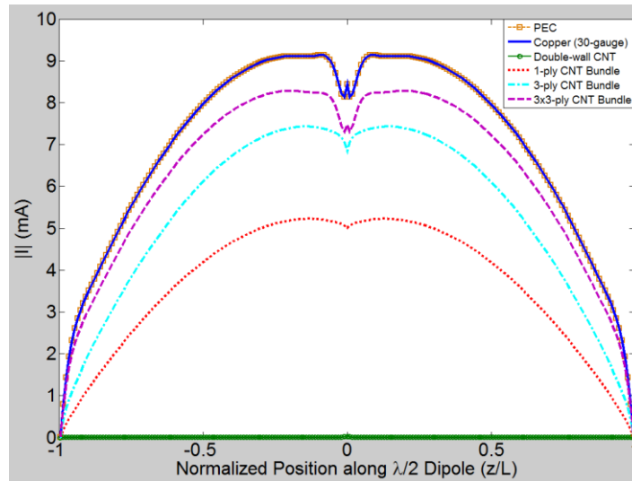
Figure 7. Comparison of current distribution (total magnitude) along \lambda/2 dipole antenna composed of different materials ( f_0 = 50 GHz, L = 3 mm).
