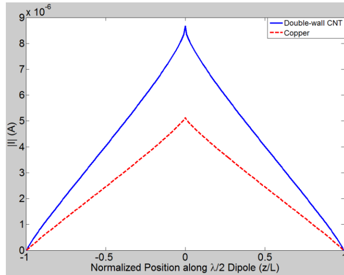
Figure 8. Comparison of current distribution (total magnitude) along \lambda/2 dipole antenna composed of nanoscale materials ( f_0 = 50 GHz, L = 3 mm).
