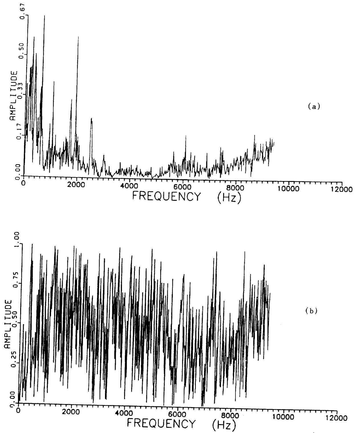
Figure 7.4 (a) Transfer function and (b) coherence function, between noise (microphone no. 1) and vibration at the operating speed of 3,000 rpm
