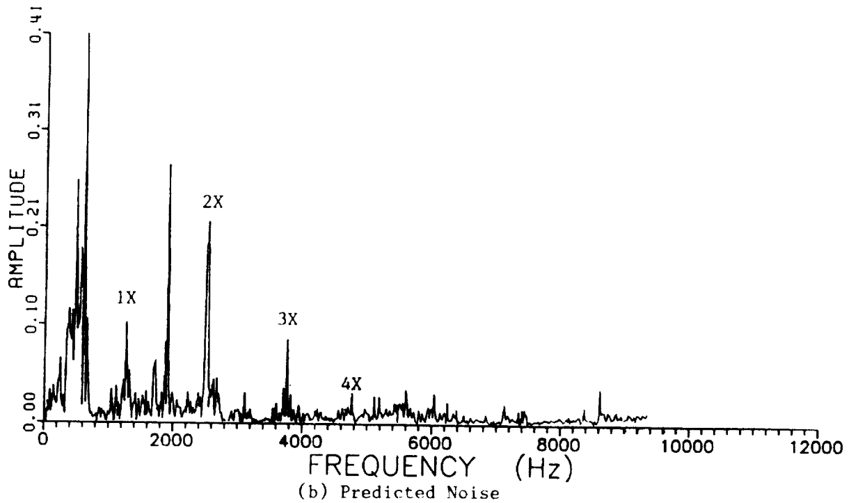
Figure 7.19 Frequency spectra of (a) experimental noise data, and (b) predicted noise results from microphone no. 1 at the operating speed of 3,000 rpm.
