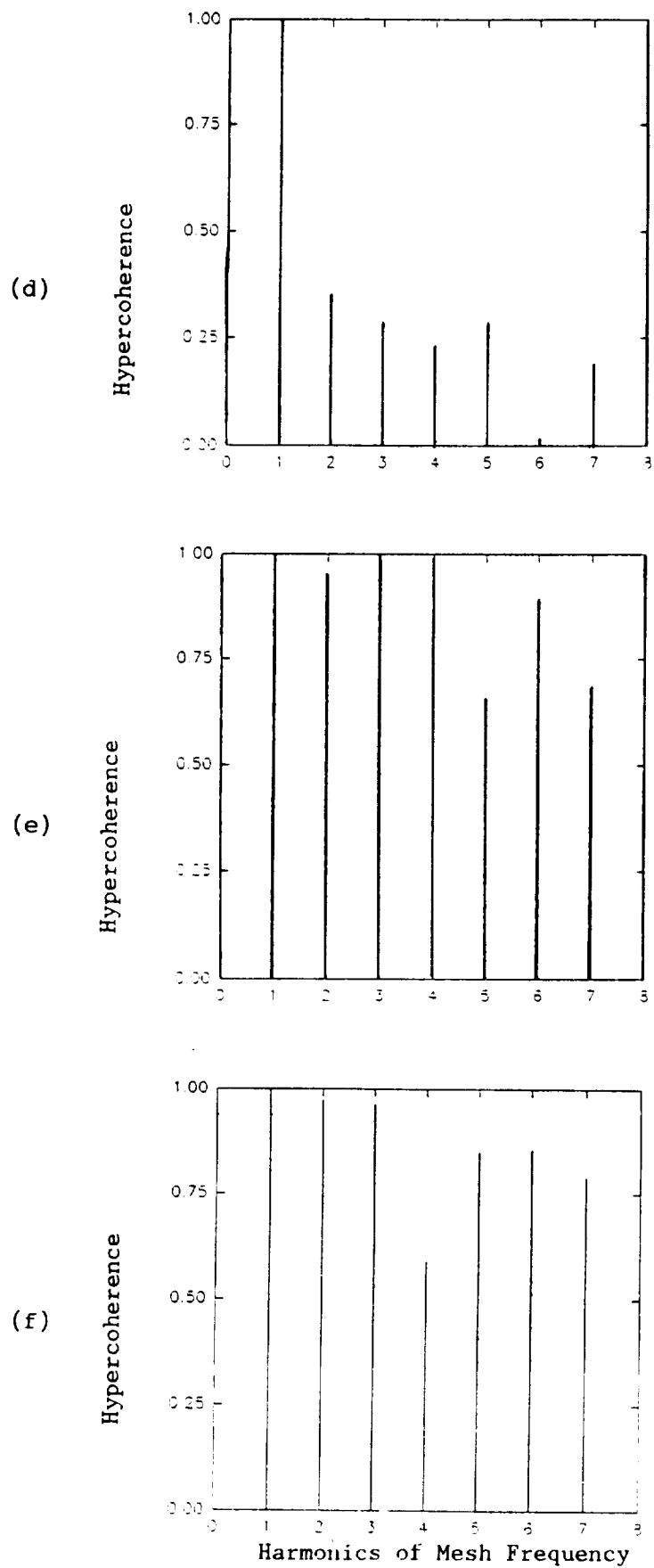
Figure 7.15 Hypercoherence function for the noise signal from microphone no. 2 (d) at 3,000 rpm, (e) at 4,000 rpm, and (f) at 5,000 rpm
