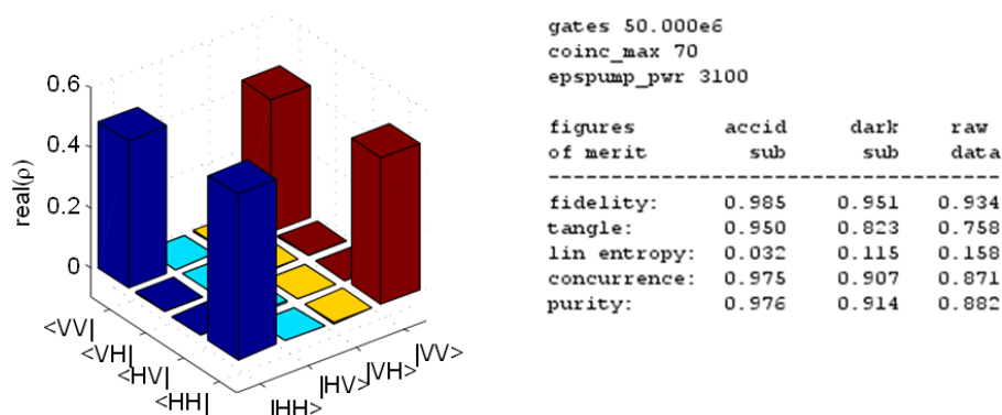
Fig. 4 Plot of the density matrix describing the quantum state of the photon pairs generated by the EPS. Various parameters are displayed in the table to show the entanglement of the photon pairs generated by the EPS.
