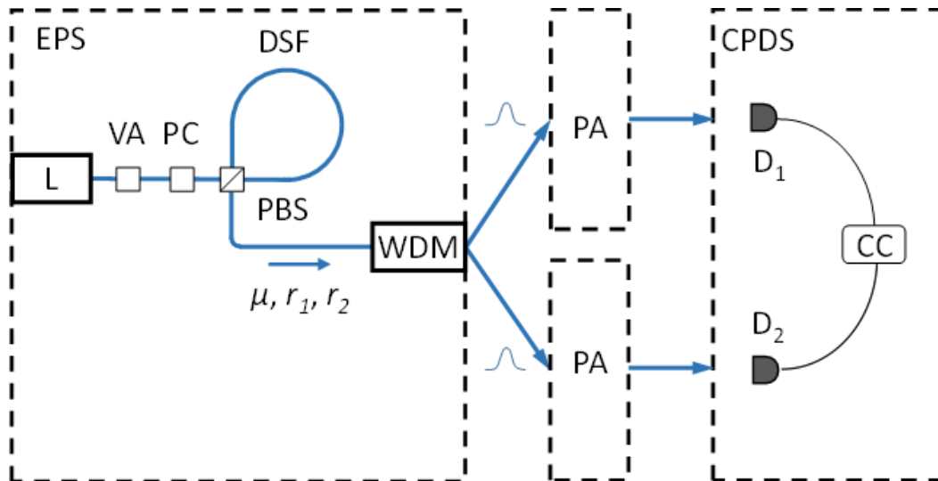
Fig. 1 Diagram of experiment setup, which includes wavelength-division multiplexer (WDM) and coincidence counting (CC) electronics
