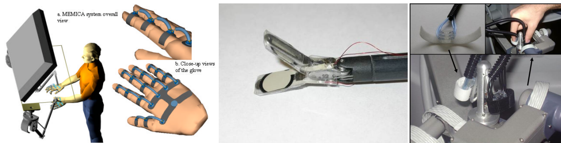
Figure 2: (left) Electro-rheological fluid (ERF) based haptic surgeon hand interface (Bar-Cohen et al., 2001); (center) Force transducer fitted to endoscopic grasper; (right) Pneumatic haptic finger tip display (Culjat et al., 2008) integrated with da Vinci ® hand controllers.
