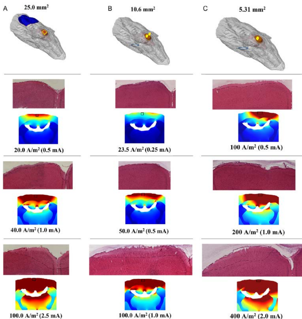
Figure 1. Microscope images (4X) of H&E stained coronal sections from tDCS-induced brain lesion and current distribution at or near -2.5 mm Bregma. Increasing tDCS current increases brain lesion in the rat as well as computationally regardless of electrode size (A, B, C). The anode (red) was placed on the skull, while the cathode (blue) was placed on either the back or chest. A. Using a 25.0 mm 2 electrode, a minimum electrode current density of approximately 20.0 A/m 2 induces cortical lesion beginning in the medial superficial cortex, which spreads laterally and penetrates into the cortex as the electrode current density is doubled. The 2.5 mA stimulation group showed a lesion was greater laterally and penetrated further into the cortex compared to the lower stimulation groups. B. Cortical damage begins to appear in the medial superficial cortex with a 0.25 mA (electrode current density: 23.5 A/m 2 ) stimulation using a 10.6 mm 2 electrode. The lesion area is also greater when the current intensity is increased. C. Using a 5.3 mm 2 electrode, lesion began to appear at 0.5 mA (electrode current density: 94.2 A/m 2 ) beginning in the motor cortex and expanded as the current intensity was increased. (For interpretation of the references to color in this figure legend, the reader is referred to the web version of this article.).
