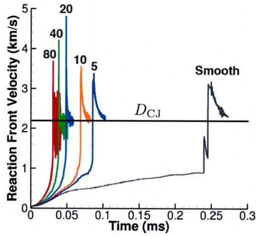
Figure 8. Summary of time to DDT for the smooth wall compared to roughness of various heights over the bottom surface. Roughness heights (5, 10, 20 40, 80) are in microns. D_{CJ} is the equilibrium detonation velocity.
