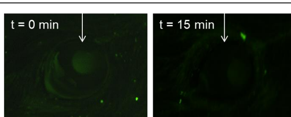
Figure 14. Rapid clearance of doxycycline delivered as topical eye drop formulation in mice. The nanowafer was instilled at t=0.
