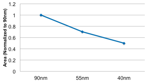
Figure 5. Embedded Flash Area Scaling (normalized)
