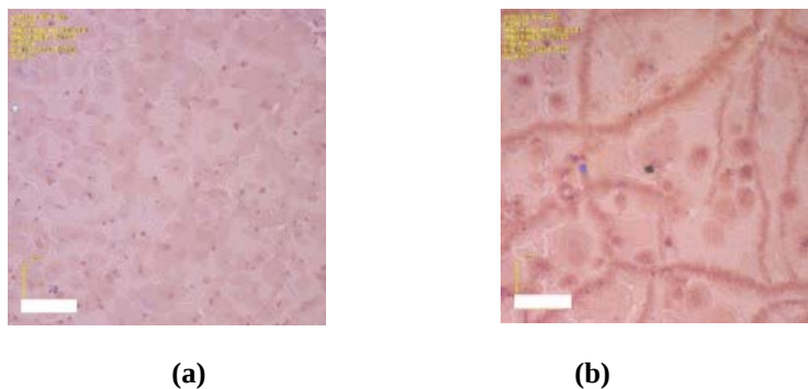
Fig. 8 Optical image of graphene transferred to a host \text{SiO}_2/\text{Si} substrate from a) metal film and b) metal foil. The scale bar represents 20\text{ }\mu\text{m} .
