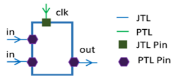
Figure 22. A template for the logic part of a standard cell that implements a 2-input Boolean gate.
