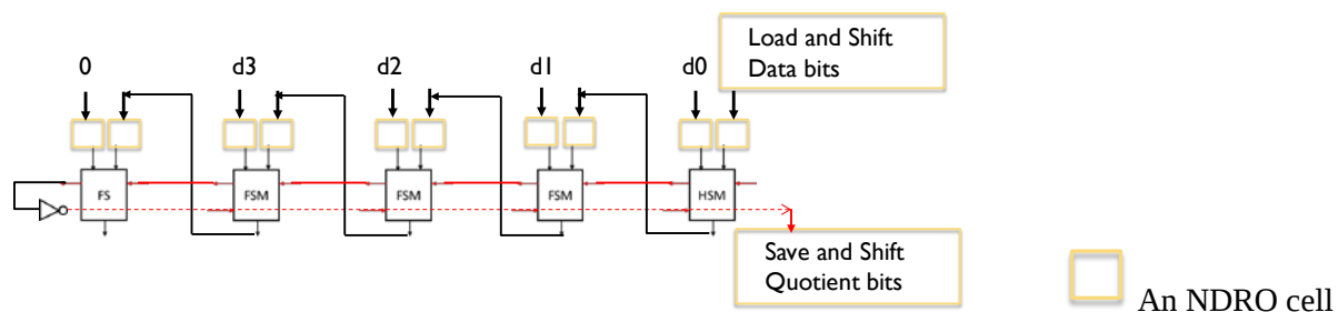
Figure 16. Bit-serial implementation of the 4-bit integer divider. HSM: Half Subtractor with Multiplexer; FS: Full Subtractor; FSM: FS with Multiplexer.
