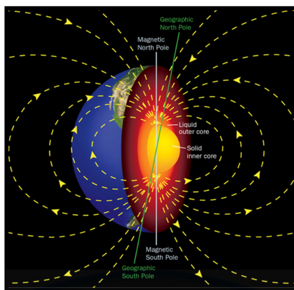
Figure 1. The Earth's Geomagnetic Field.
