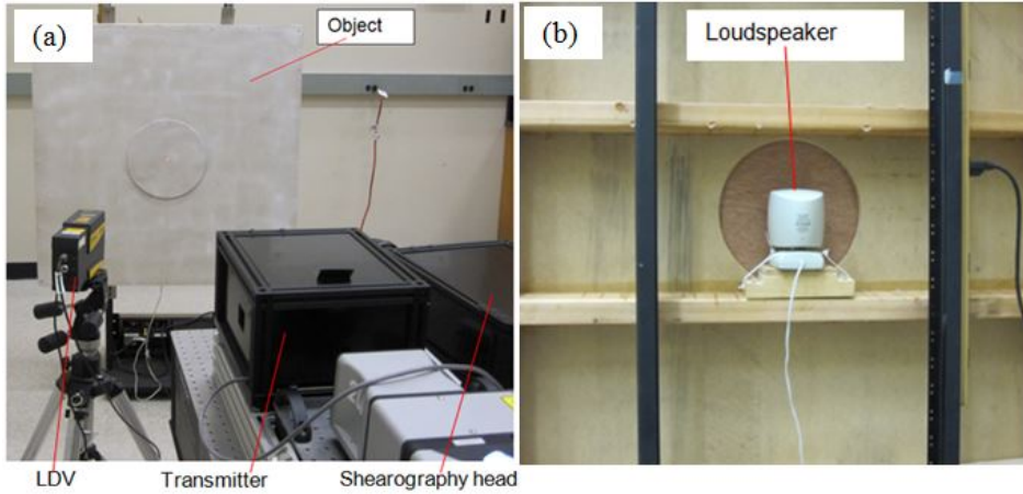
Figure 4. Photographs of the experimental setup for taking shearograms of a vibrating object (a), and a loudspeaker mounted behind the object (b).
