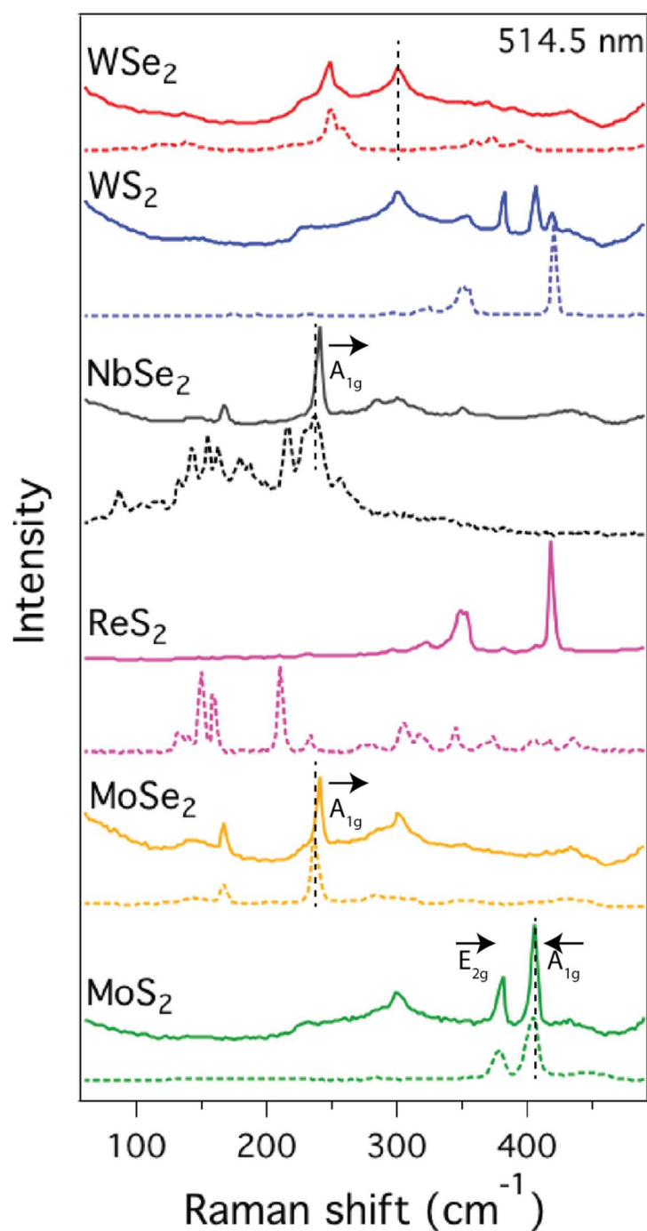
Figure S10. Raman spectra of few layer and bulk TMDs. MoS 2 shows characteristic shifts in the A 1g – E 2g energy levels (~ 2 cm -1 ) due to reduction in thickness (black dotted line). Similar shifts are seen in NbSe 2 , MoSe 2 , as well as new low-dimensional modes appearing in MoSe 2 and WSe 2 . These data suggest reduction of dimensionality in exfoliated TMDs compared to bulk powders.
