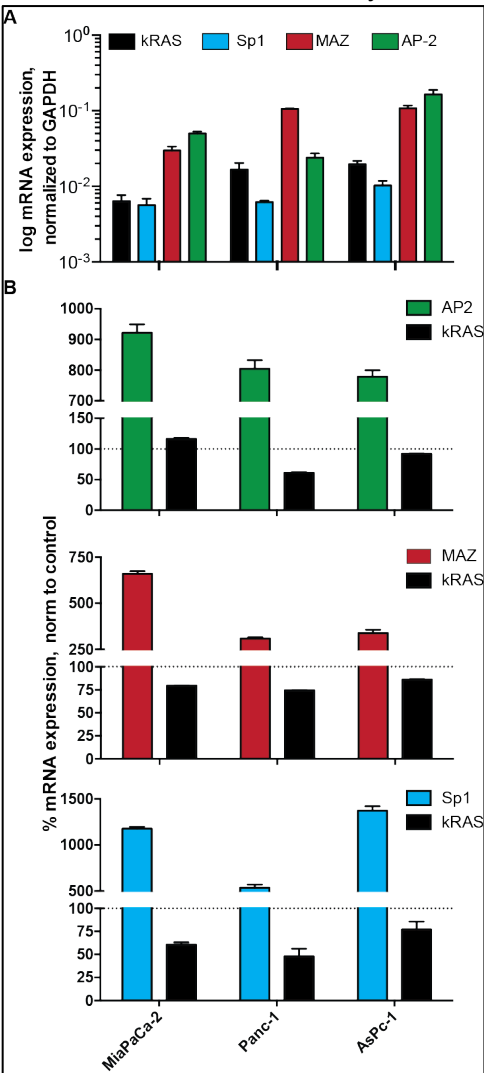
Figure 15. Increased kRAS promoter activity by transcription factors. (A) The cell lines vary in the basal expression of each of the proteins of interest, as shown by internal normalization to GAPDH. (B) Plasmids encoding for AP-2 (top), MAZ (middle) and Sp1 (bottom) were transfected into the pancreatic cancer cells such that their expression went up 3 – 15-fold. The effects of MAZ and Sp1 overexpression on kRAS transcription was consistent with the luciferase findings; AP-2 effects varied per cell line, leading to a significant increase in MiaPaCa-2 cells and a significant decrease in Panc-1 cells. No change was noted in AsPc-1 cells. n=3 for all experiments, with qPCR technical duplicates.
