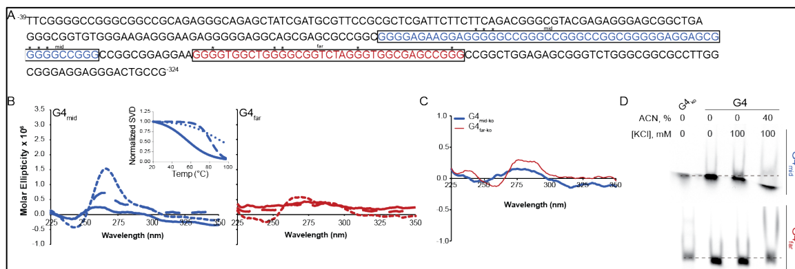
Figure 1. G4 formations in the extended kRAS promoter region. (A) The kRAS promoter shown from - 324 to - 39 bp relative to the transcriptional start site, contains distinct guanine-rich regions, termed near, mid, and far in the 5'–3' direction; only mid- and far-were considered for this study; * denote G-to-T mutations within each region for knockout mutations shown in (C). (B) ECD was used to determine G4 formation and stability within each of these G4-forming regions in the absence (solid line) or presence of 100 mM KCl alone (long dash line) or in the presence of 40% acetonitrile (ACN) (short dash line). Thermal stability from 20 to 100 °C is shown in the inset of mid; the lack of strong G4 formation for G4 far made melting not possible. (C) ECD demonstrated a lack of inducible G4 formation in the presence of 100 mM KCl with the selected G-to-T mutations in the knock-out (ko) sequences. (D) Electromobility shift assays were used to demonstrate the inter- versus intra-molecular G4 formations within each G4-forming region in the presence of 100 mM KCl with or without 40% ACN. A downward shifting of the DNA with the G4 mid sequences, as compared to its linear ko sequences, indicates intramolecular structure formation, particularly evident in the presence of both cationic strength and dehydration. The G4 far sequence, in the absence and presence of 100 mM KCl, demonstrates a downward shift from the linear ko sequence, but there is no difference between these two solvent conditions. In contrast, in the presence of KCl and ACN, there is a lack of a downward shift and the presence of retarded migration, as compared to control and KCl alone, indicating the potential for intramolecular G4 species.
