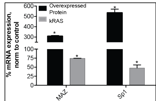
Figure 13. MAZ and Sp1 downregulate kRAS transcription in PANC-1 cells. Plasmids encoding for MAZ and Sp1 were transfected into PANC-1. Both proteins significantly decreased kRAS transcription, consistent with the luciferase findings. * p < 0.05 as compared to control; n = 3 individual experiments, each run in duplicate with qPCR duplicates of each sample.
