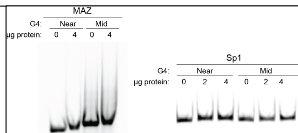
Figure 11. The binding of MAZ and Sp1 to FAM-labeled Near- or Mid-G-quadruplexes (as induced by 100 mM KCl) were examined. Neither protein, at concentrations up to 4 µg, demonstrated a supershift of the DNA, indicating there is no protein-DNA interaction.
