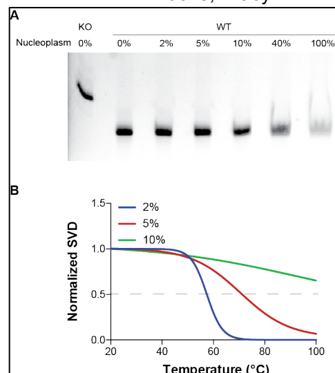
Figure 9. Effect of Nucleoplasm on G4 mid formation. (A) Incubation with increasing amounts of nucleoplasm maintains an intramolecular G4 structure, although the pattern becomes diffuse with more equilibrating structures at 40 and 100%. (B) The effect of 2-10% nucleoplasm on G4 thermal profiles was examined. Thermal stability increases with more nucleoplasm, consistent with (A), but the number of isoforms is fewest at 2%.
