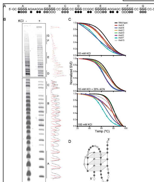
Figure 5. Predominant G4 isoforms formed within the mid-region of the kRAS promoter. (A) The G4 mid sequence has seven runs of continuous guanines, A–G. The circles indicate evidence of protection in the subsequent DMS footprinting: light gray circles indicate marked protection, medium gray indicate partial protection, and black circles indicate DMS-mediated piperidine cleavage. (B) DMS footprinting of the mid promoter region of kRAS in the presence (+) or absence (-) of 100 mM KCl was performed. Images obtained from the top and bottom portions of the sequencing gel (boxed individually) were aligned, Image J software was used to graph and align histograms of the guanine cleavage pattern (no KCl = black line; 100 mM KCl = red line). (C) Thermal stability of a series of G-to-T mutants interrupting runs A–G, individually, of the G4 mid sequence in the presence of 10 mM KCl alone (top), in the presence of 20% ACN (middle), or with 100 mM KCl (bottom). (D) Cumulatively, these data predict a G4 isoform formation of a tri-stacked structure incorporating runs B, C, E and F with intervening loops of 2, 10, and 8 bases in the 5'–3' direction. G = black circles, C = dark gray circles, T = light gray circles, A = white circles.
