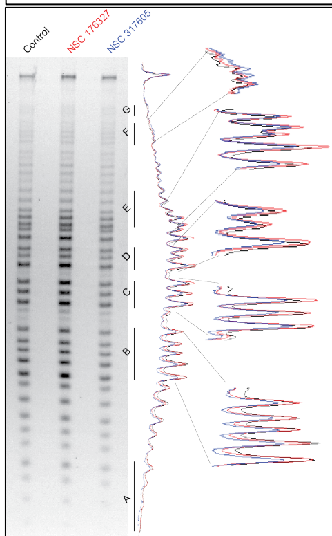
Figure 8. Varying stabilization of G4_{mid} by small molecules. G4_{mid} was incubated with 10 mM KCl alone or in the presence of NSC 176327 or NSC 317605 at 2.5 equivalences, each. Histograms of the DMS labeling and cleavage are shown on the right, with expanded sections of runs B-F.
