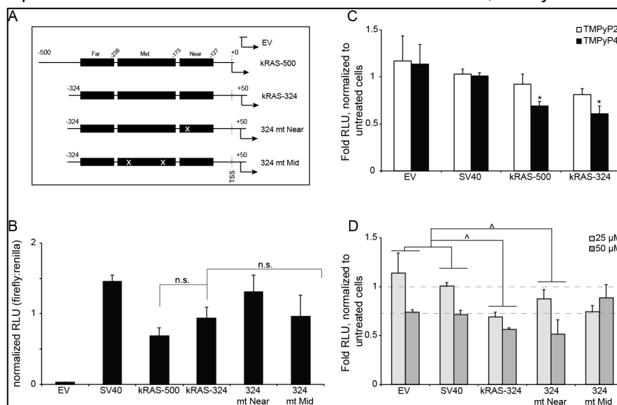
Figure 2. Isolating silencing G4 formations within the KRAS promoter. (A) A series of luciferase plasmids were constructed from the promoterless empty vector (EV) pGL4.17 backbone to localize the silencing G4s within the KRAS promoter. These included KRAS -500 (-500 – +0, relative to the transcriptional start site (TSS)), and KRAS -324 (-324 – +50 relative to the TSS). Site-directed mutagenesis of KRAS -324 was used to introduce G-to-T mutations (approximate location indicated with white x) that abrogate G4 near (324 mt Near) or G4 mid (324 mt Mid) formation. (B) Basal expression of the non-mutated plasmids was examined in transiently transfected HEK-293 cells for 48 hr and normalized to renilla expression in co-transfection assays. Promoterless (EV) and constitutively active (SV40) plasmids were included as comparison. There was no significant difference between the KRAS promoter plasmids. (C) The effects of HEK-293 treatment (48 hr) with 25 \mu M TMPyP2 and TMPyP4 on promoter activity was examined in the EV, SV40 and wild-type KRAS promoter containing plasmids KRAS -500 and KRAS -324. TMPyP4 was equally significant ( ^{\#}p < 0.05 as compared to untreated control, per plasmid, as determined by one-way ANOVA) in lowering promoter activity in the two KRAS promoter plasmids, whereas it was inactive in the non-G4-containing EV and SV40 plasmids at that concentration. TMPyP2 was also inactive in all plasmids. (D) A TMPyP4 dose response (25 and 50 \mu M) was performed in the wild-type KRAS -324 plasmid and its two generated mutant plasmids 324 mt Near and 324 mt Mid. The dose response was performed in the non-G4-containing EV and SV40 plasmids. The colorimetric contribution of 50 \mu M TMPyP4 is evident in the EV and SV40 containing plasmids. In all plasmids where a dose-response was evident, the magnitude of that response was examined by a two-way ANOVA. Both KRAS -324 and 324 mt Near maintained significant ( ^{\wedge}p < 0.05 for dose response, as compared to EV and SV40 effects) G4-mediated silencing of promoter activity, whereas 324 mt Mid did not. These findings indicate that G4-mediated silencing is contained within the mid-guanine-rich region of the KRAS promoter. All experiments were performed in a minimum of triplicate.
