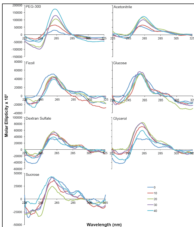
Figure 4. Dehydrating and Crowding co-solvent effects on G4 mid formation. 0 – 40% of varying co-solvents were incubated with the DNA during the G4-annealing process. Spectral effects were measured and the percentile of each co-solvent saturating its effect was determined to be 10% for Glucose, 20% for Ficoll, Glycerol, Sucrose, Dextran Sulfate and ACN, and dual effects with PEG-300 at 20% and 40%.
