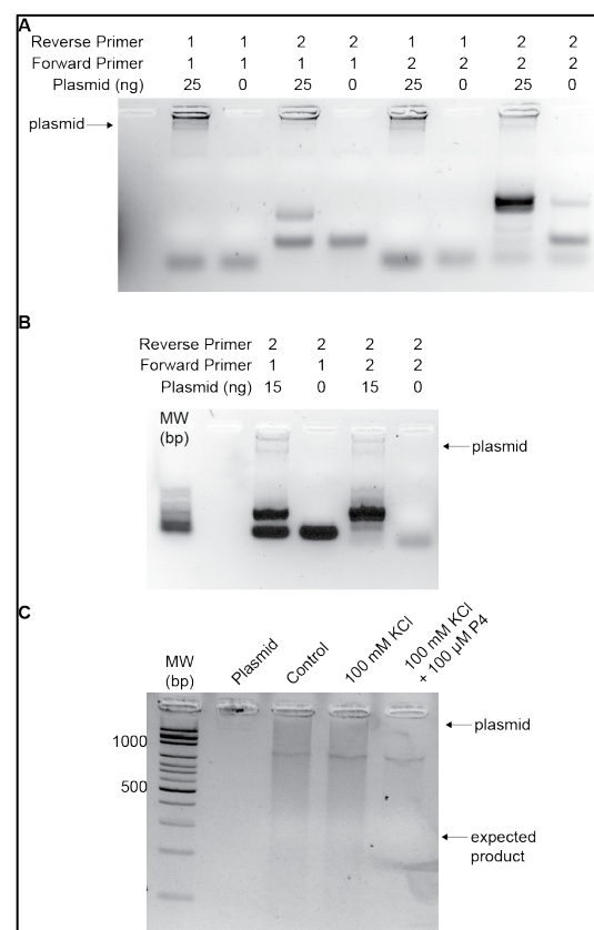
Figure 16. Primer optimization for plasmid DMS footprinting. (A) Two forward and two reverse primers were designed to amplify the G-rich region of the KRAS promoter and were tested in all four possible combinations with 25 ng of plasmid. (B) The two conditions with Reverse primer 2 were examined with 15 ng of plasmid to enhance product formation and decrease primer dimer. F2/R2 primers were deemed optimal. (C) KRAS-324 plasmid was incubated in buffer alone, with 100 mM KCl or with 100 mM KCl + 100 μM TMPyP4 before amplification with the F2/R2 primer pair. Larger than expected PCR products were identified (950 vs the anticipated 250 bp).
