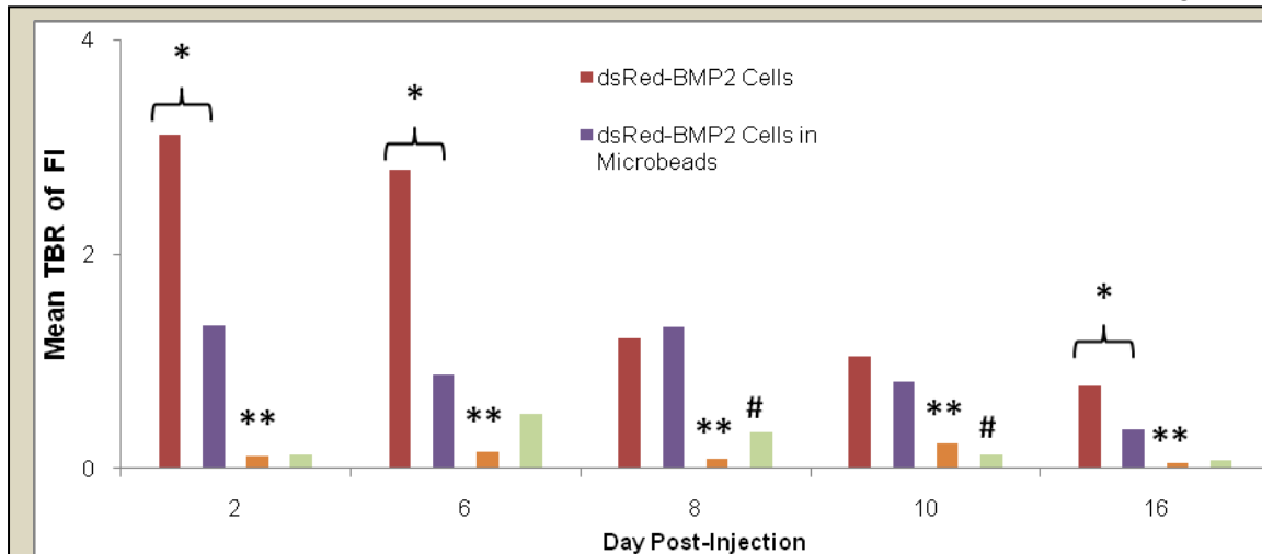
Figure 4: Mean Target-to-Background Ratio (TBR) of Fluorescence Intensity (FI) in mice given unencapsulated dsRed cells, microencapsulated dsRed cells or microencapsulated control cells. *P < 0.05 for Ad5dsRED-BMP2 transduced cells versus Ad5dsRED-BMP2 cells in microbeads at days 2, 6, and 16 post-injection. **P < 0.05 for Ad5dsRED-BMP2 cells transduced cells versus Ad5dsRED-BMP2 cells in microbeads at all time points. # P < 0.05 for dsRED-BMP2 cells in microbeads versus Ad5empty cassette transduced cells (Control) in microbeads at days 8 and 10 after injection.
