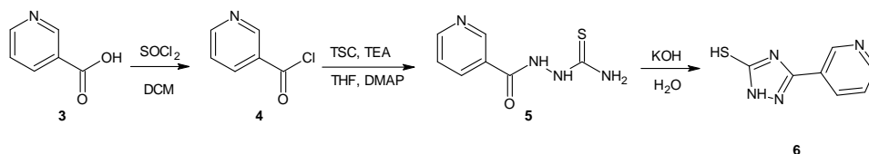
Scheme 2. Synthesis of triazole heterocycle 6
