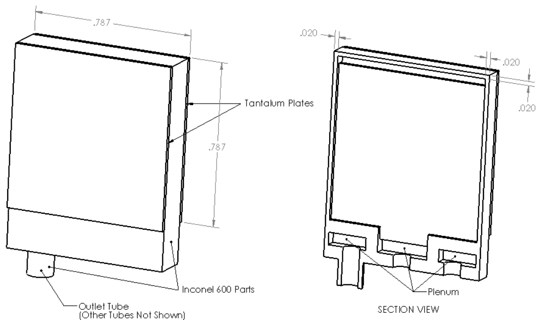
Fig. 4 MR 2.1.4 (dimensions in inches)
