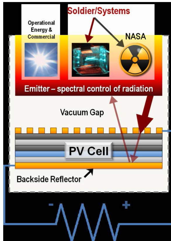
Fig. 1 Primary components of the TPV energy converter 1
