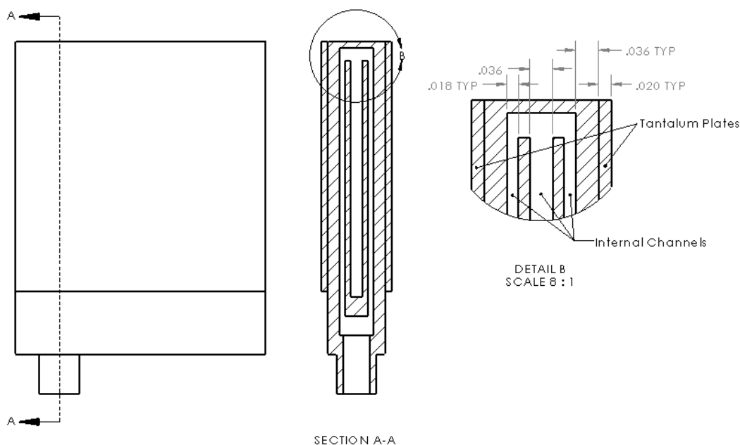
Fig. 5 MR 2.1.4 detail view (dimensions in inches)
