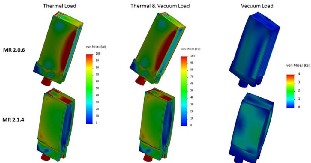
Fig. 9 MR 2.0.6 and MR 2.1.4 stress
