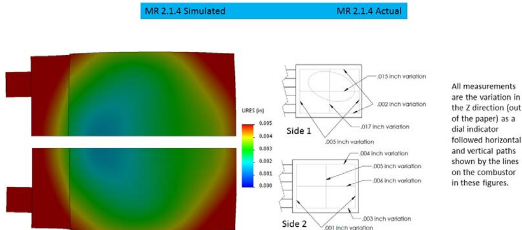
Fig. 18 Comparison of simulated and measured deformation of MR 2.1.4 due to thermal load only
