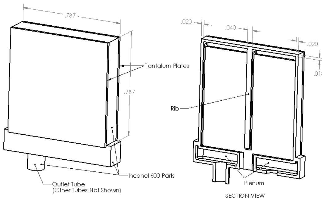
Fig. 2 MR 2.0.6 (dimensions in inches)
