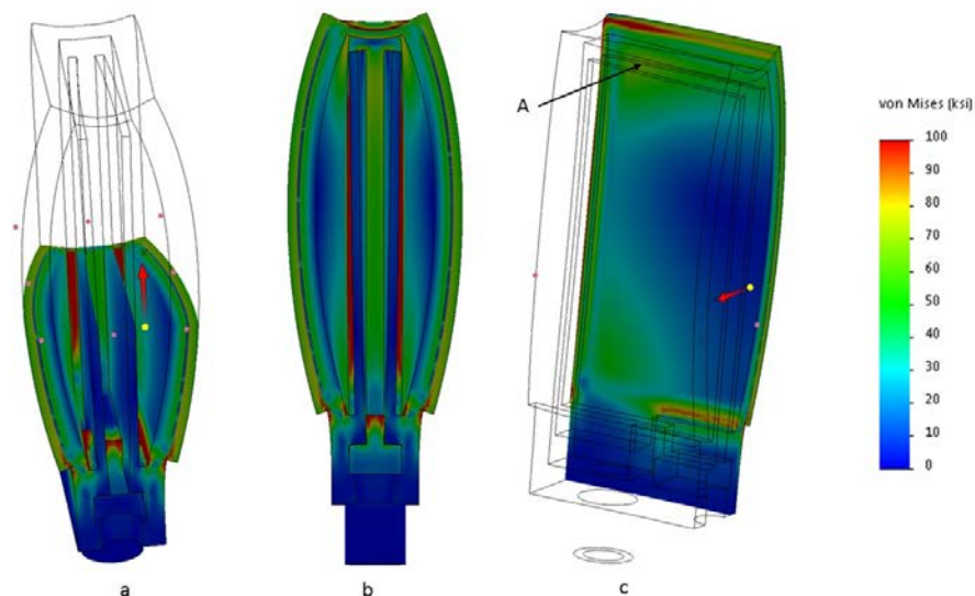
Fig. 13 MR 2.1.4 stress due to thermal load cross sections
