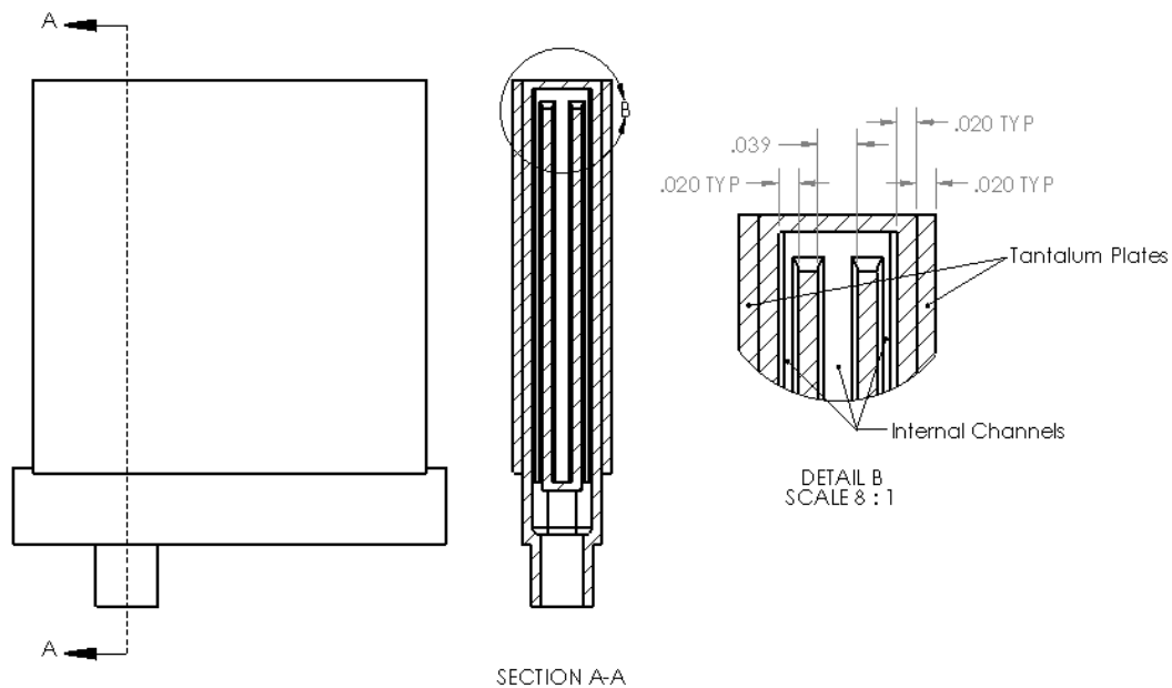
Fig. 3 MR 2.0.6 detail view (dimensions in inches)
