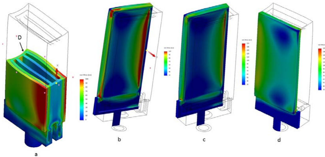
Fig. 11 MR 2.0.6 stress due to thermal load cross sections
