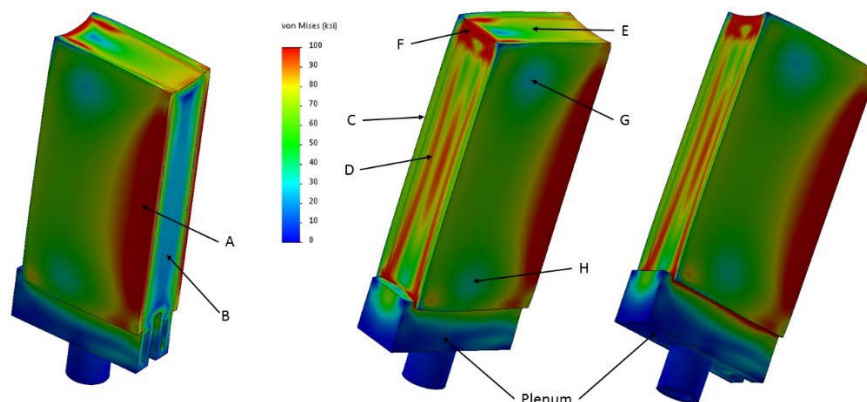
Fig. 10 MR 2.0.6 stress due to thermal load
