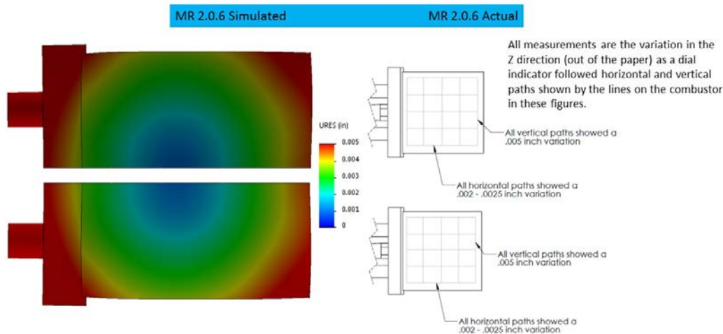
Fig. 16 Comparison of simulated and measured displacement of MR 2.0.6 due to thermal load only
