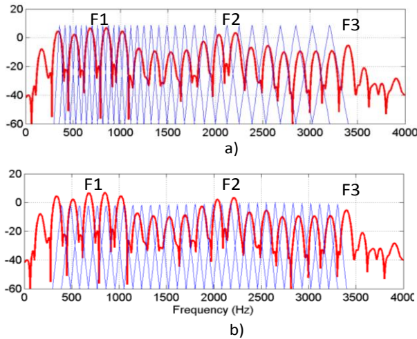
Fig. 2. An example of speech spectrum overlapped with A) Mel filterbanks, and B) Linear filterbanks.
