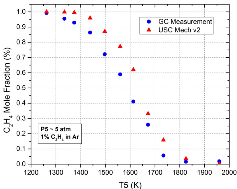
Figure 4: Ultimate ethylene mole fraction - GC measurement vs. USC Mech v2 (1% C 2 H 4 /Ar, P5 ~5 atm)
