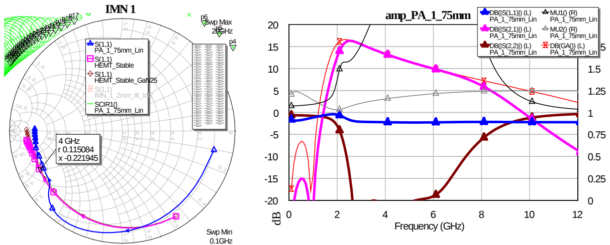
Fig. 9 Stabilizing resistors added to 10- × 175-μm GaN HEMT (28 V) plus broadband output match
