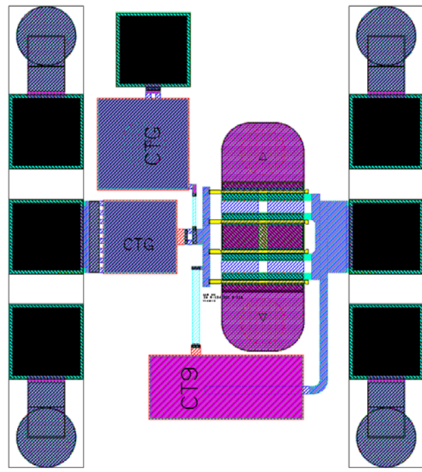
Fig. 49 Layout plot of stand-alone broadband feedback amplifier (0.6 × 0.6 mm)
