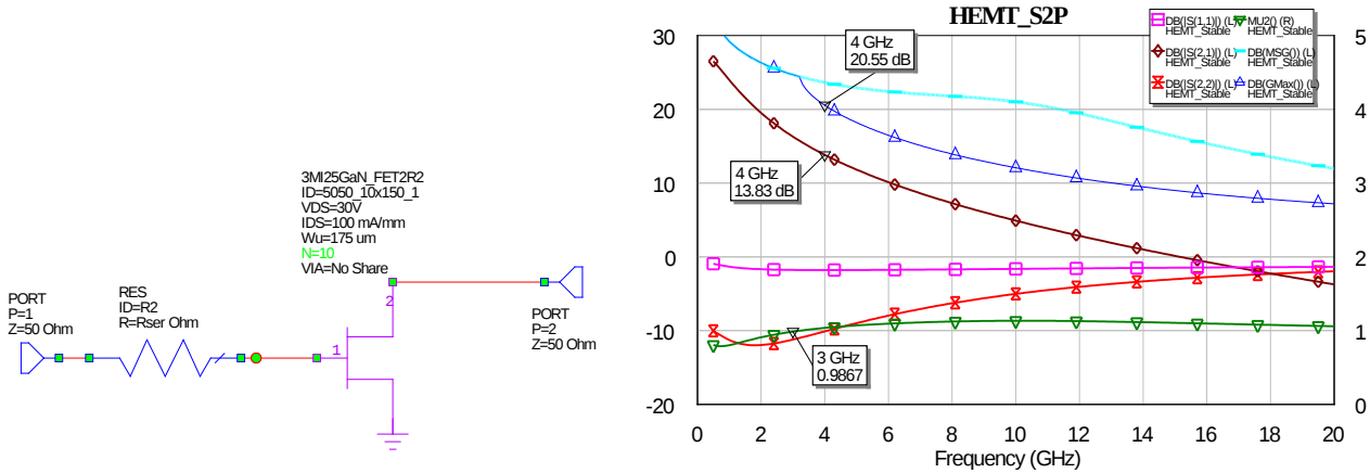
Fig. 8 MWO S-parameter simulation of 10- × 175-μm (1.2-mm) GaN HEMT (28 V and 180 mA)
