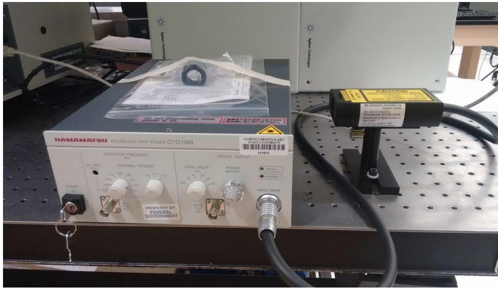
Figure 9: Hamamatsu picosecond pulsed laser system
