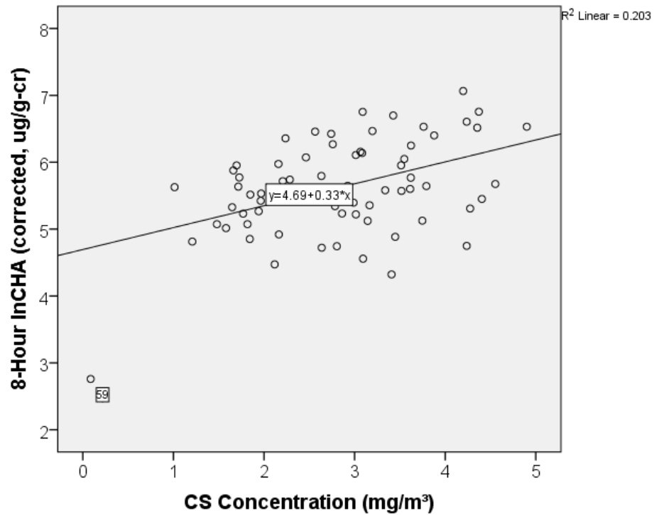
Figure 16. Relationship between CS exposure (mg/m³) and CHA levels corrected for creatinine (µg/g-cr) at the eight-hour sample interval
