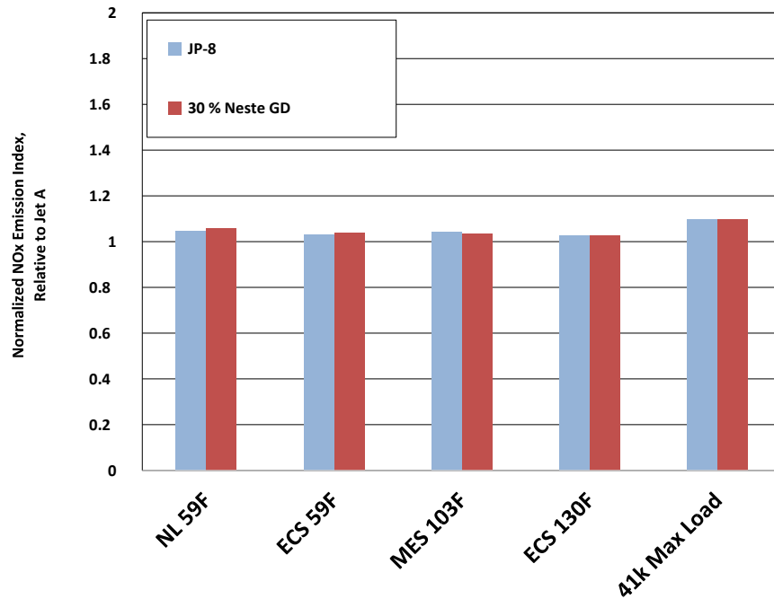
Figure 7. 131-9 Rig NOx Relative Emissions.
