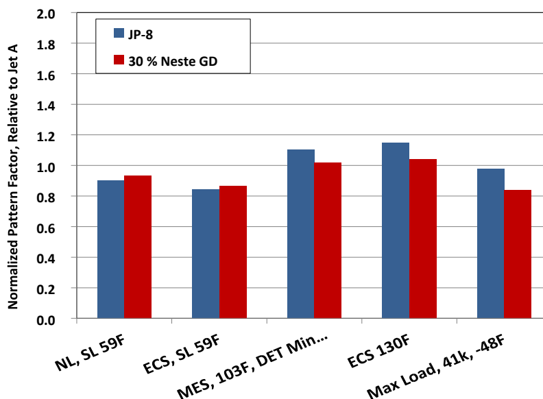
Figure 5. 131-9 Combustor Relative Pattern Factor.
