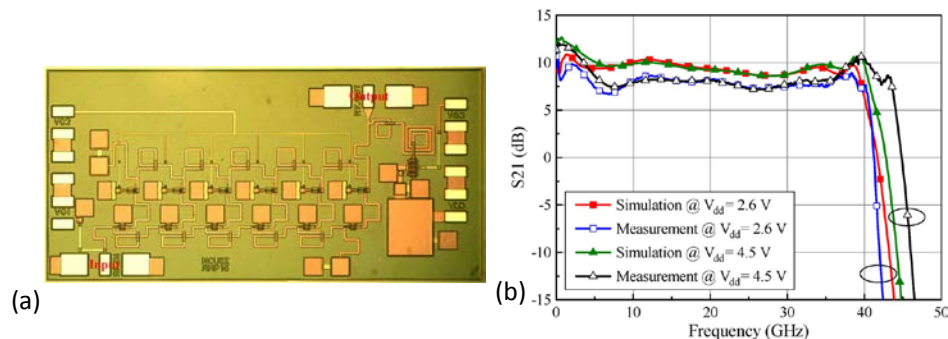
Figure 23: (a) Photograph of the six-stage HEMT-HBT cascode distributed amplifier chip (b) Simulated and measured small-signal gains [37].
