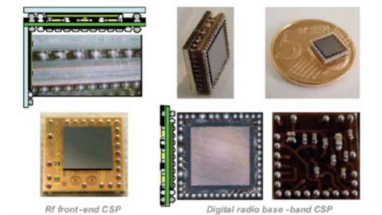
Figure 87: Fully integrated low power RF radio, measuring 7x7x2.5 mm 3 , realized by 3D stacking of WLP (CSP) packages [133].
