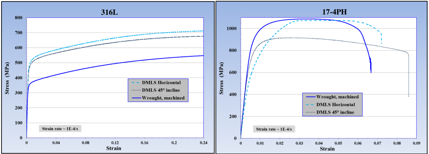
Figure 9: Measured room-temperature tensile deformation behavior of stainless steels produced with DMLS, compared to that of annealed, wrought and machined material.
