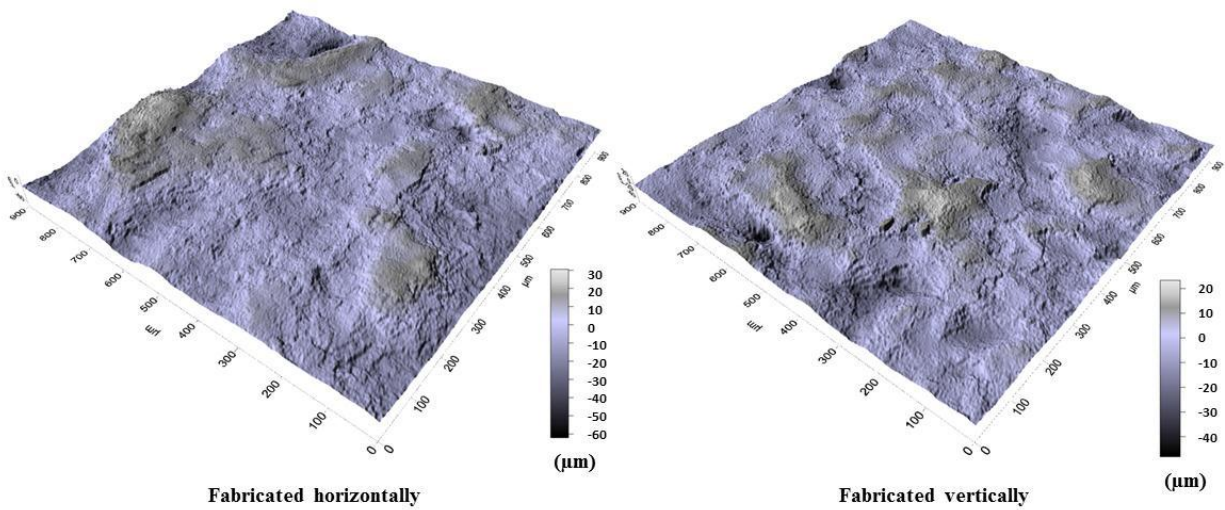
Figure 3: Surface maps from optical profilometry of DMLS SS316L fatigue specimens.
