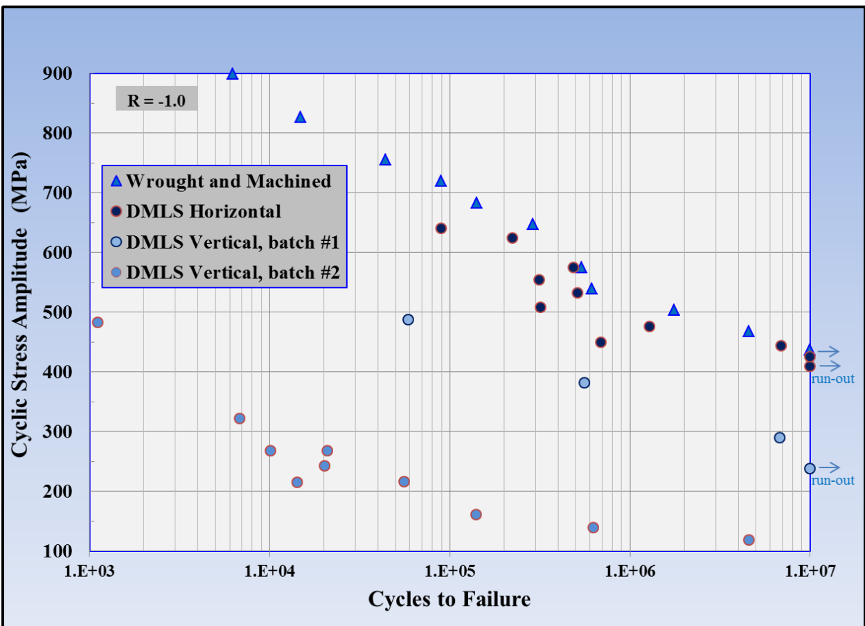
Figure 16: Measured room-temperature stress-life (S-N) of DMLS 17-4PH, compared to that of conventional material. Bending fatigue (rotating beam) at a frequency of 25 Hz.
