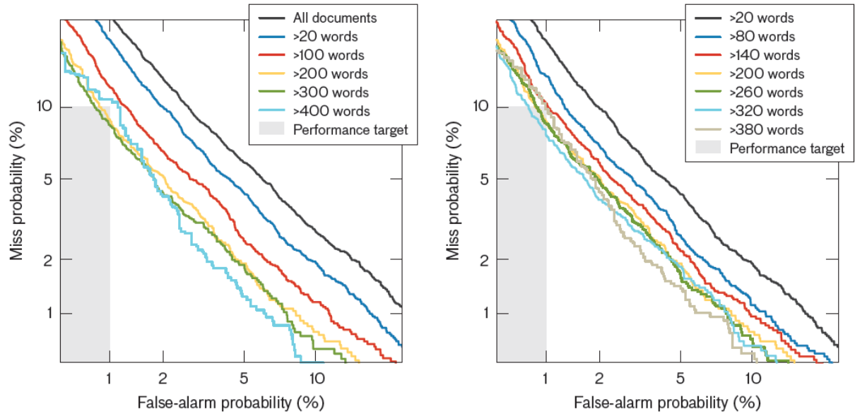
FIGURE 7. As the minimum number of words in each Reddit document is increased, the classifier's performance improves.
