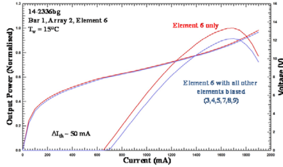
Figure 9. CW performance of element 6 with and without thermal load from adjacent array elements.
