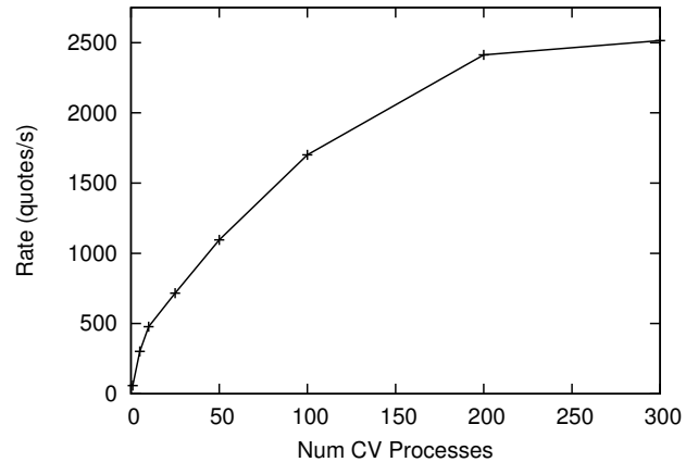
Figure 9: Scaling the CV on bare metal
