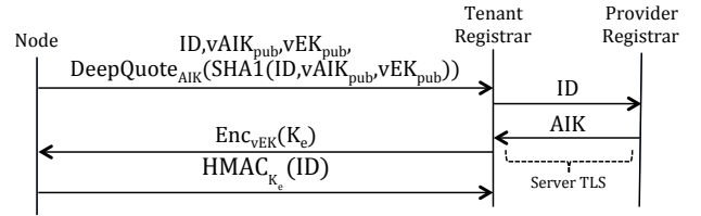
Figure 4: Virtual node registration protocol.
