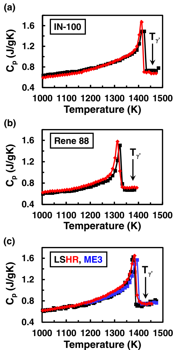
Fig. 3 On-cooling specific-heat-versus-temperature measurements for a IN-100, b René 88, and c LSHR. For IN-100 and René 88, the two sets of measurements ( black, red ) were taken approximately 9 months apart on different samples from the same billet. For LSHR, the red and black data pertain to samples from two different billets measured approx. 10 years apart. The LSHR results are compared to the behavior for the alloy ME3 (in blue ) in c
