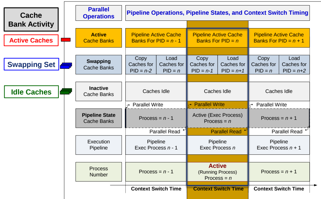
Fig. 6 OS friendly microprocessor architecture context switch timing diagram
