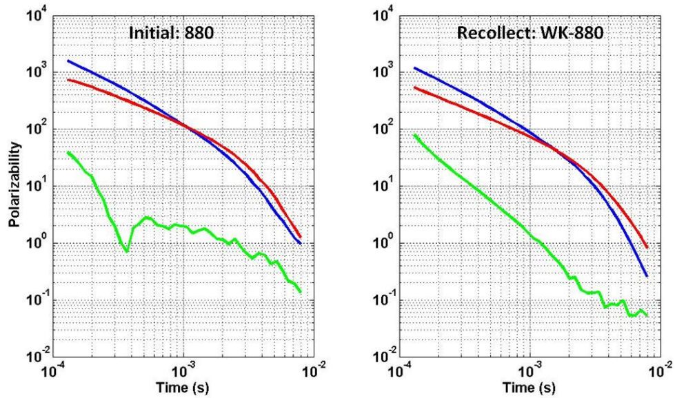
Figure 13. Polarizabilities Recovered from the Initial Acquisition Data (Left) and the Recollect Data (Right).
