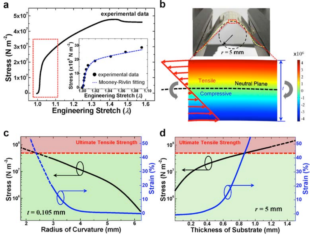
Figure 17: Computational non-linear hyperelastic analyses on the mechanical bending stress of the flexible MoS 2 TFT. (a) Measured stress( \sigma )–stretch( \lambda ) curve of the specimen of solution based PI and PET ( t = 0.105 mm). The inset shows experimental data fitted with Mooney-Rivlin model. (b) The numerical result on hyperelastic nonlinear stress analyses based on the parameters extracted from the experimental data when the bending radius is 5 mm. The top inset shows a photograph of the bent MoS 2 TFTs with a radius of 5 mm. (c-d) Based on the Mooney-Rivlin model, the expected mechanically stable range (green region) of the structure with respect to the (c) radius of curvature of the substrate and (d) thickness of the substrate.
