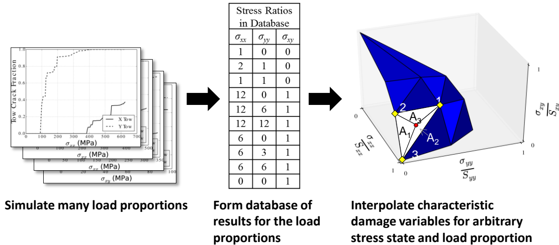
Figure 2.2.5 Reduced order model for predicting characteristic damage states
