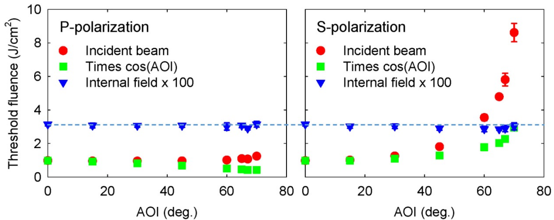
Figure 1: Dependence of ablation threshold fluence on the angle of incidence on a gold sample, for two different polarization of the laser beam (P and S). The value of internal fluence at the point of ablation threshold is independent of the angle of incidence.
