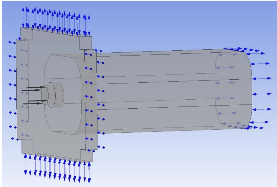
Figure 24. Boundary Conditions
