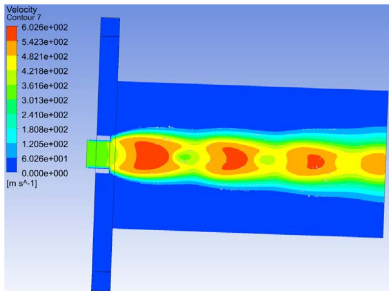
Figure 25. Velocity Contours
