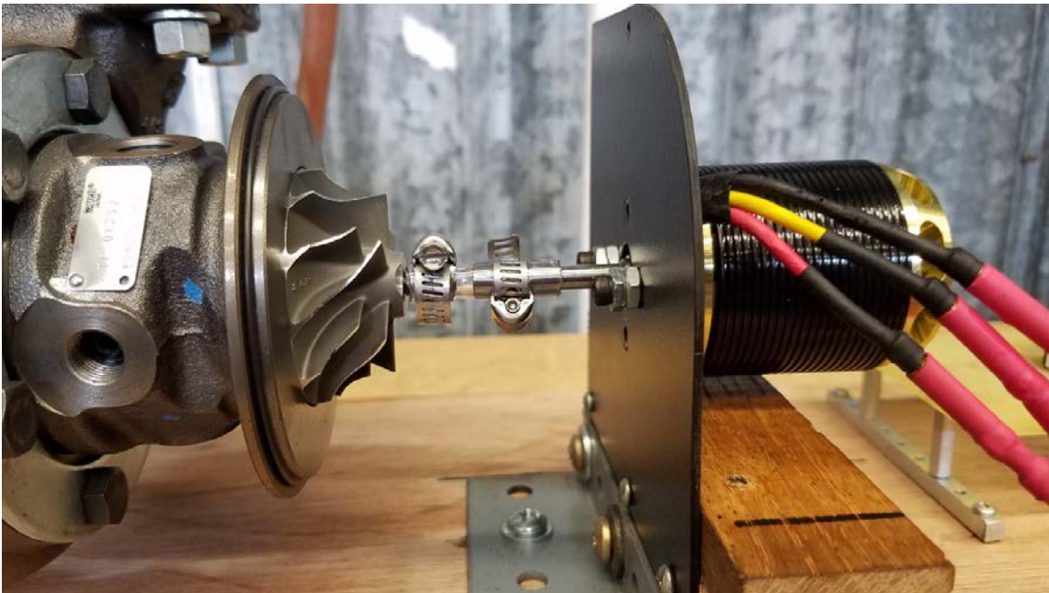
Figure 9. High Speed Flexible Coupling
