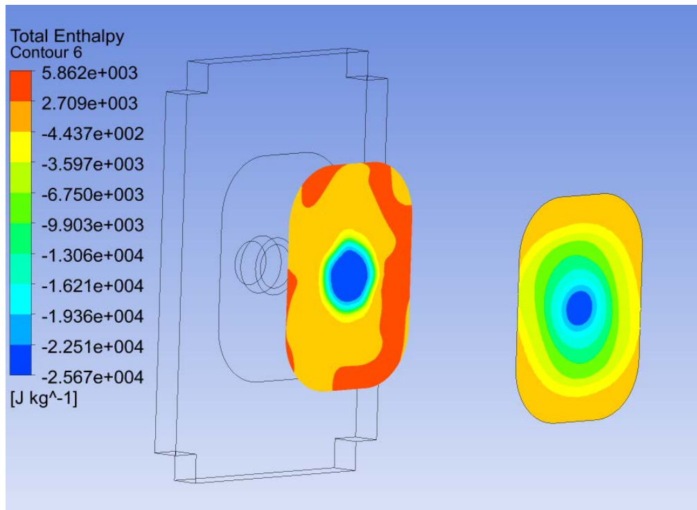
Figure 26. Total Enthalpy Contours
