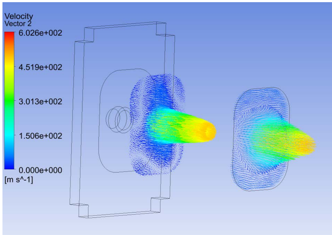
Figure 28. Velocity Vectors
