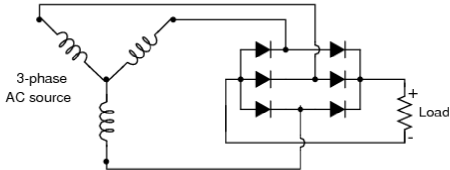
Figure 5. Three Phase Full Wave Bridge Rectifier Circuit. Source: [13].
