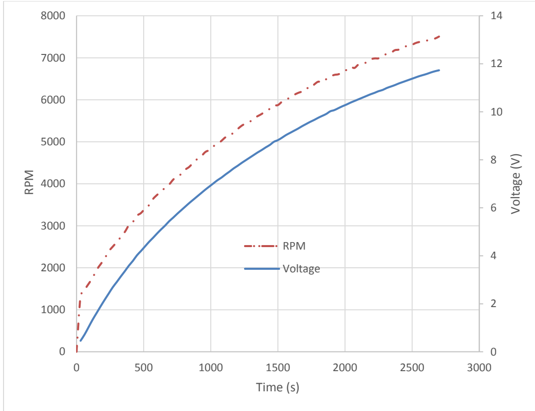
Figure 13. Curves for the Second Charging Cycle
