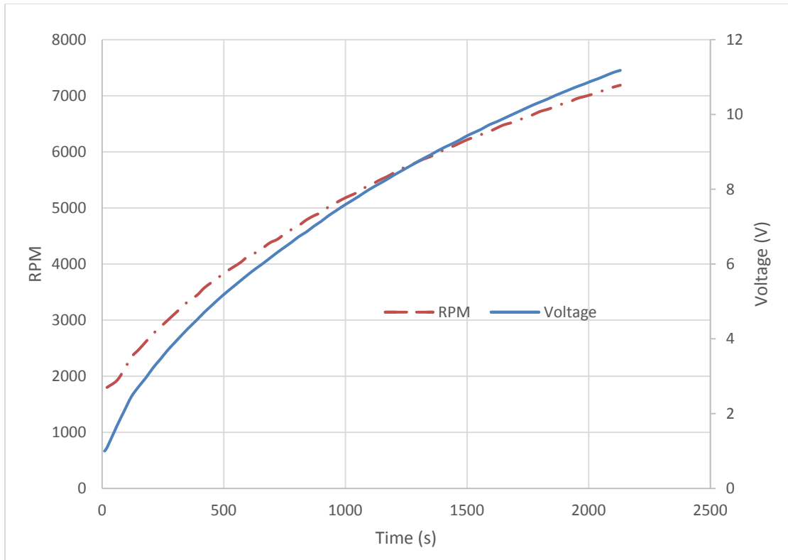
Figure 12. Curves for the First Charging Cycle
