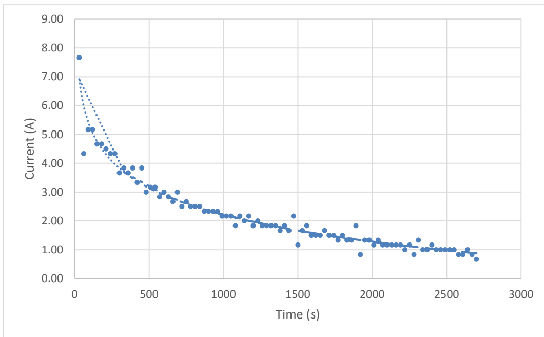
Figure 16. Current vs. Time for the Second Charging Cycle
