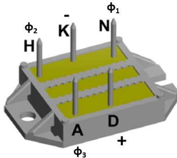
Figure 7. Rectifier Chip with Labeled Leads. Adapted from [15].
