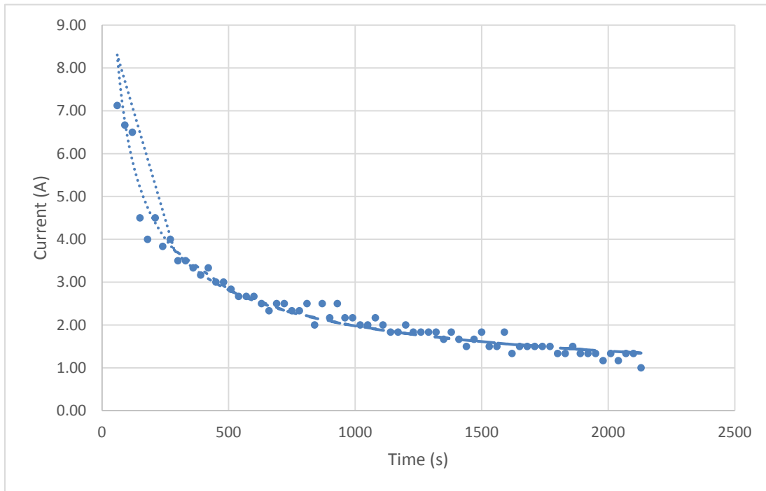
Figure 14. Current vs. Time for the First Charging Cycle
