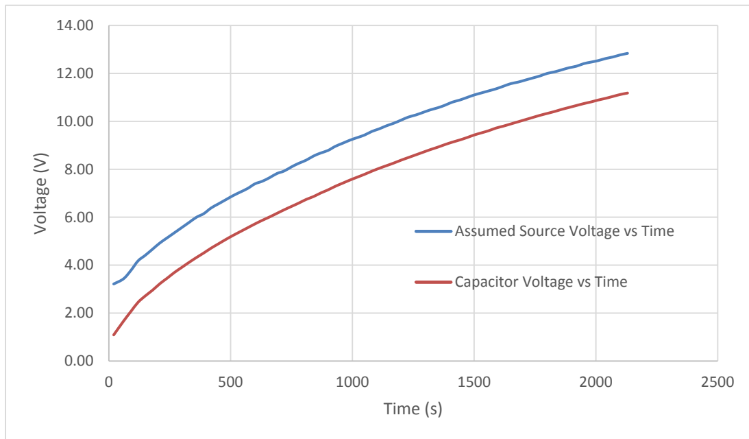
Figure 20. Comparison of Assumed Source Voltage and Recorded DC Voltage
