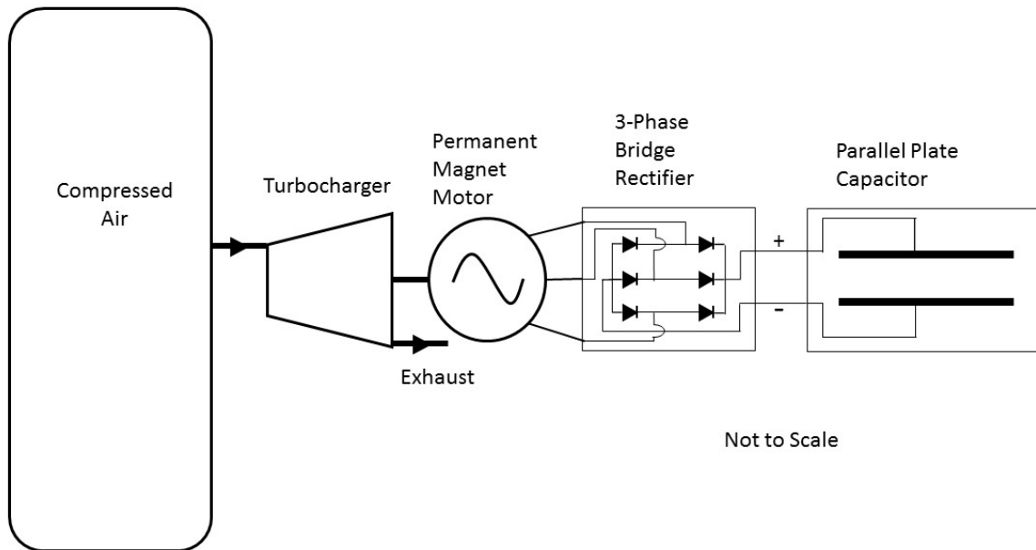
Figure 1. Proposed Design Concept
