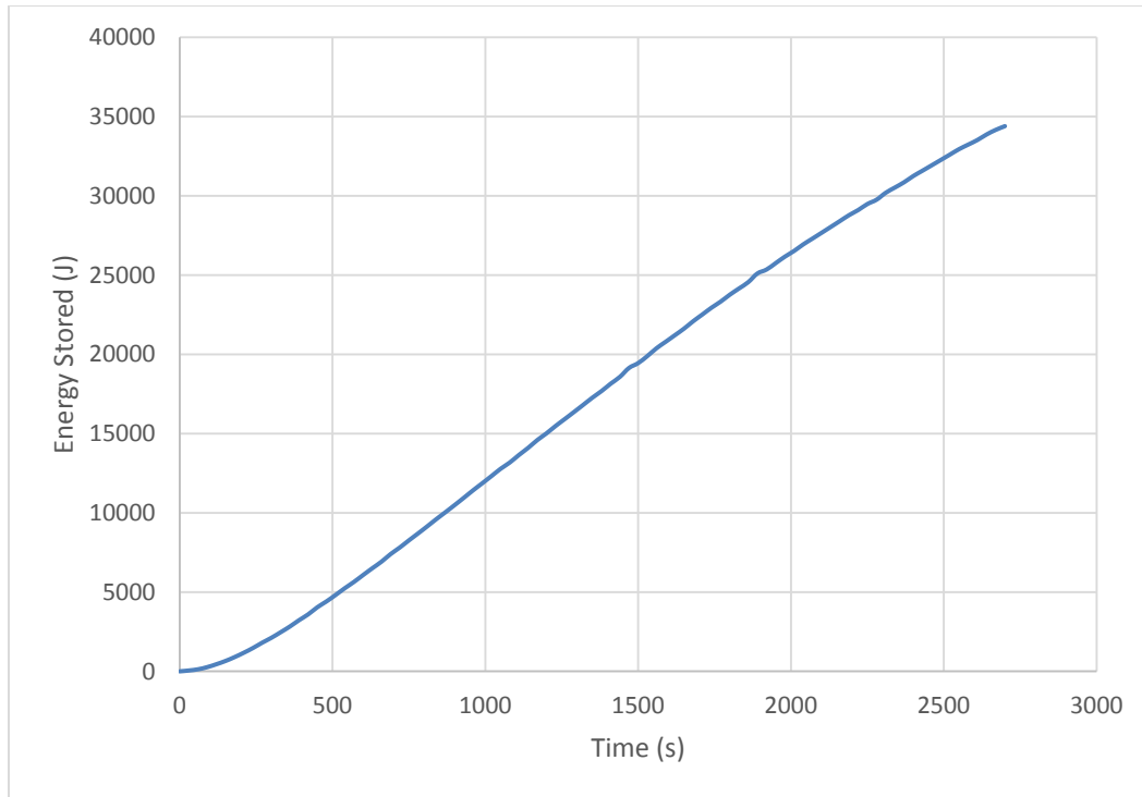
Figure 17. Energy Stored vs. Time for the Second Charging Cycle
