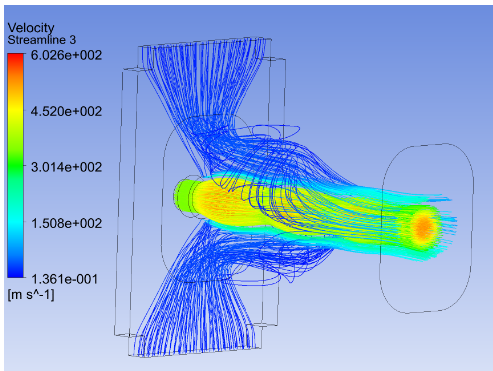
Figure 27. Streamlines from Inlet and Two Openings
