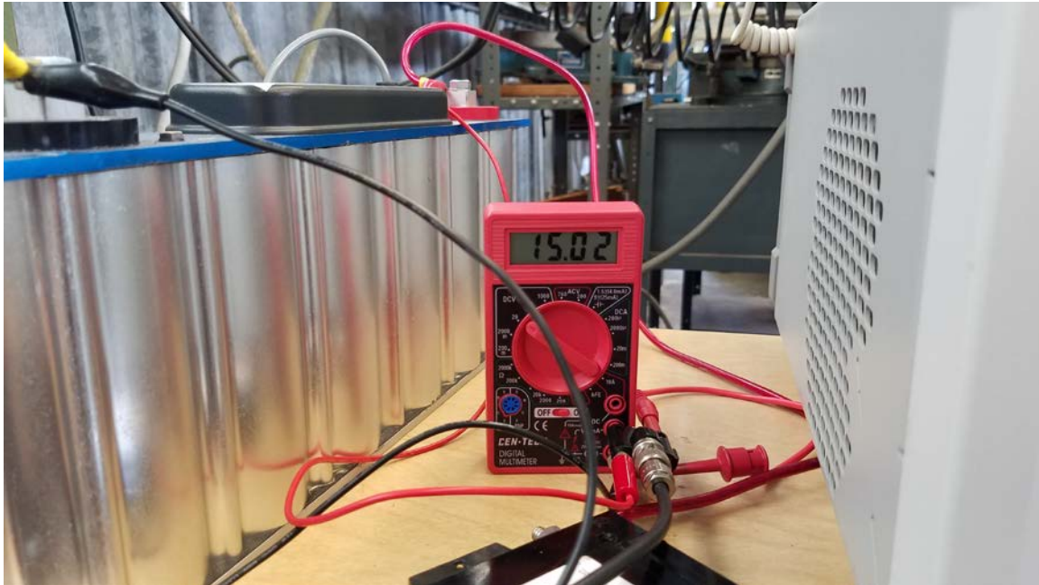
Figure 18. Final DC Voltage across the Capacitor
