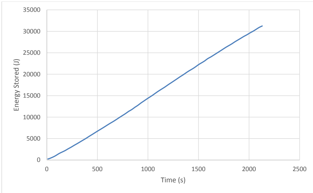
Figure 15. Energy Stored vs. Time for the First Charging Cycle
