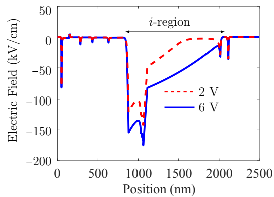
Fig. 7: The calculated electric field in the device at 2 and 6 V.
