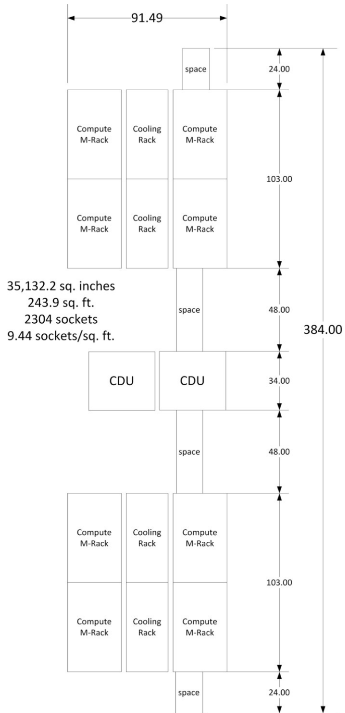
Figure 6.11-1: Base Case SGI ICE X M-Cell Maximum Density Layout
