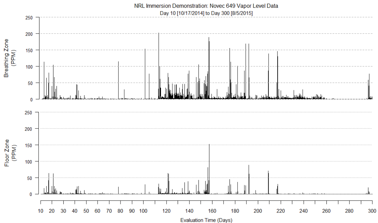
Figure 6.4-1: Breathing Zone Vapor Concentration Compared to Floor Zone Vapor Concentration During Normal Operation
