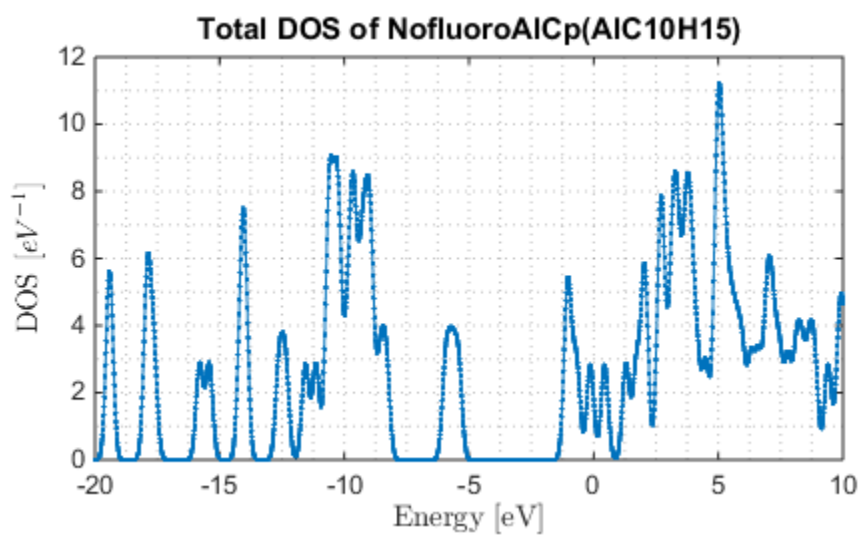
Figure 27. Total DOS for \text{AlC}_{10}\text{H}_{15}
