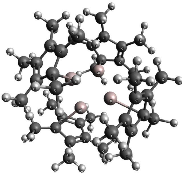
Figure 8. Tetramer \text{Al}_4\text{C}_{40}\text{H}_{60}
