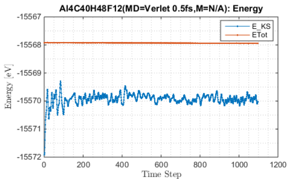
Figure 29. Total energy conserved with MD=Verlet, and length of time step at 0.5 fs
