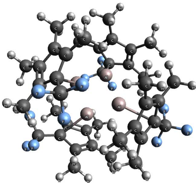
Figure 7. Tetramer \text{Al}_4\text{C}_{40}\text{H}_{48}\text{F}_{12}
