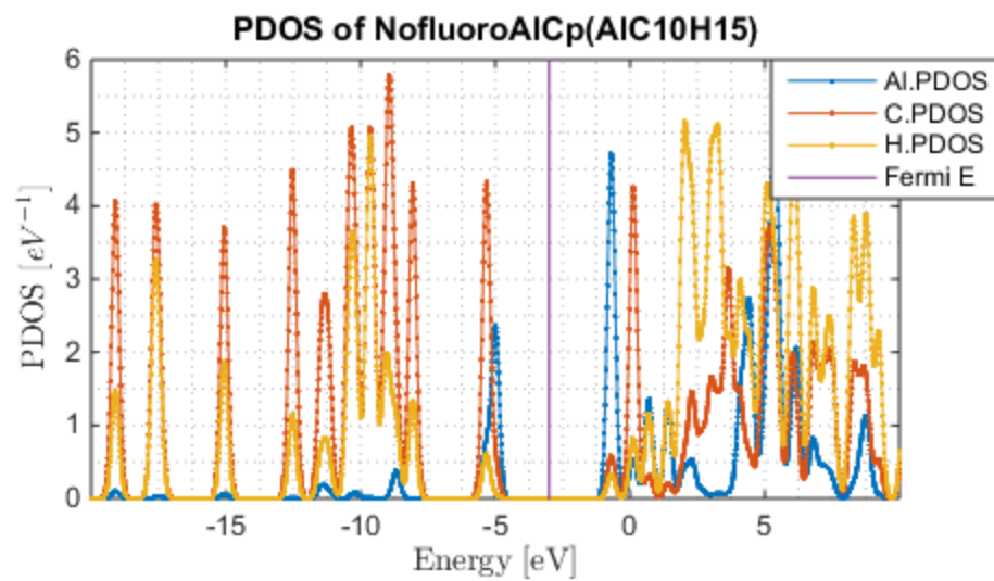
Figure 26. PDOS for \text{AlC}_{10}\text{H}_{15}
