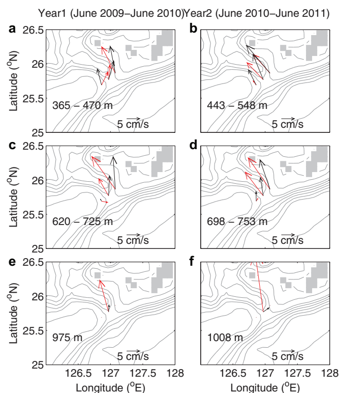
Fig. 2. Mean current vectors at upper (a, b), middle (c, d), and near sill depth (e, f) layers in Kerama Gap for year-1 (left) and year-2 (right) at CM1 (southwest) to CM3 (northeast). Only CM2 has measurements near the sill depth. Observations from Na et al. (2014) are shown in black and the HYCOM reanalysis in red. Gray represents model land points. The reference vector is shown in the lower right corner of each panel. (For interpretation of the references to color in this figure legend, the reader is referred to the web version of this article).
