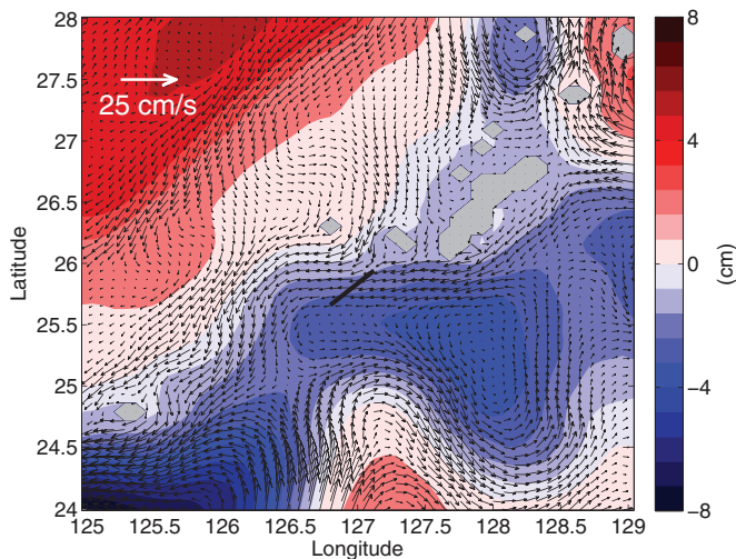
Fig. 9. SSH difference (year-2–year-1, cm) and layer-1 velocity difference (year-2–year-1, cm/s) between year-2 (June 2010–June 2011) and year-1 (June 2009–June 2010) from the global HYCOM reanalysis.
