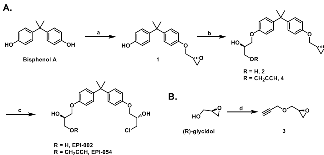
Scheme 1. Synthesis of EPI-002 and EPI-054. a
