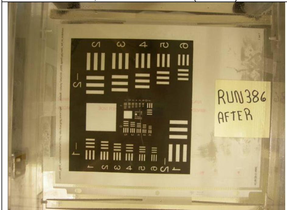
OCTAFLO EF @ -20°C, Nominal% \text{H}_2\text{O} Reduction, 4mm Initial Fluid Thickness, After 10 min Run Time (Run #386)
