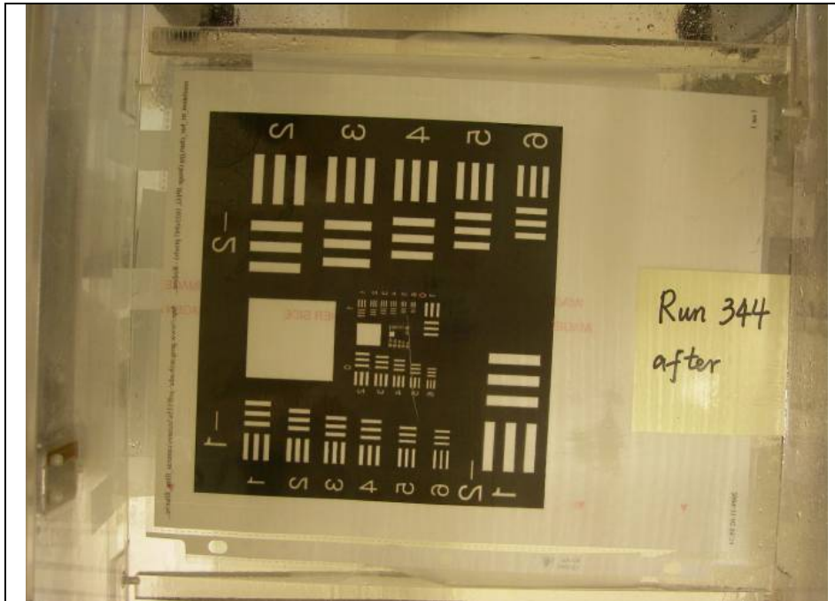
OCTAFLO EF @ -20°C, Nominal% \text{H}_2\text{O} Reduction, 4mm Initial Fluid Thickness, After 10 min Run Time (Run #344)
