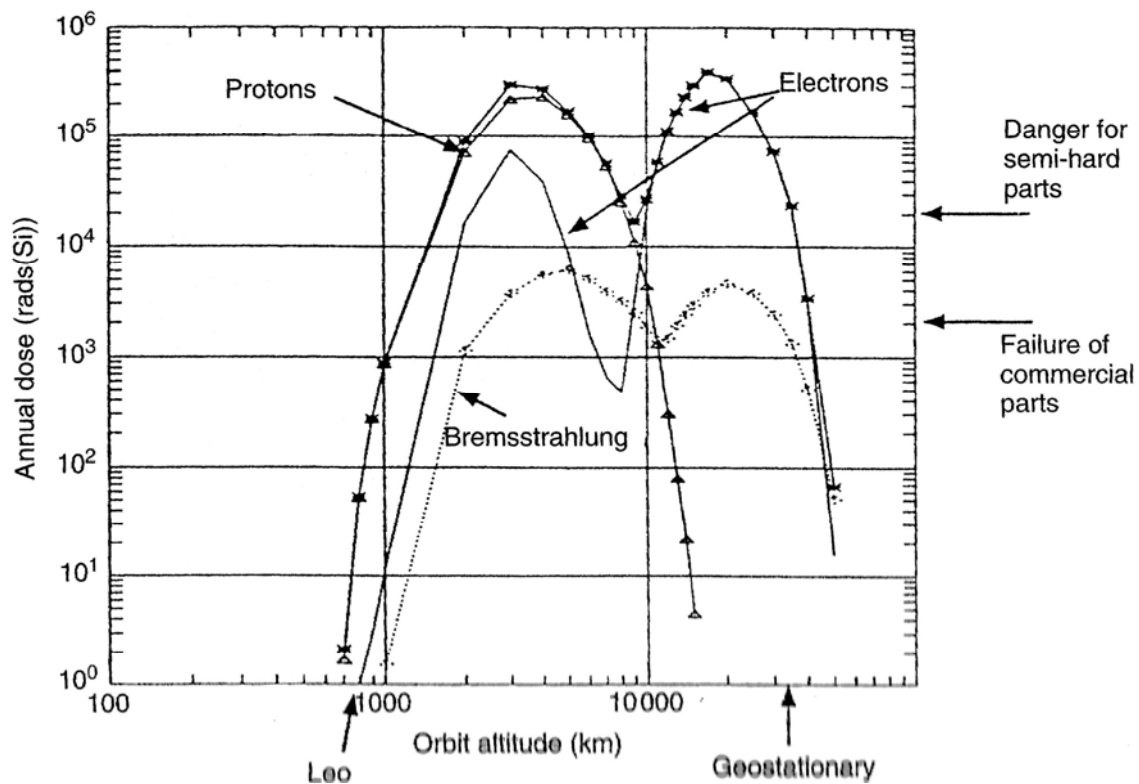
Figure 16. The Structure of the Van Allen Radiation Belts. Source: Fortescue, Swinerd, and Stark (2011, 30).
