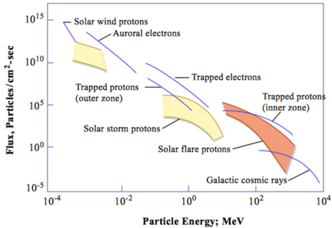
Figure 18. Particle Flux and Particle Energy. Source: MIT OCW (2006).
