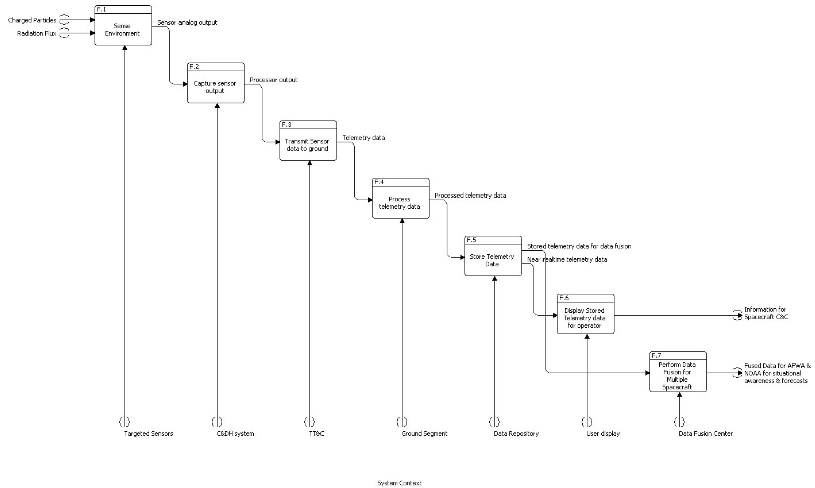
Figure 30. IDEF0 Model for Targeted Space Environment Monitoring.
