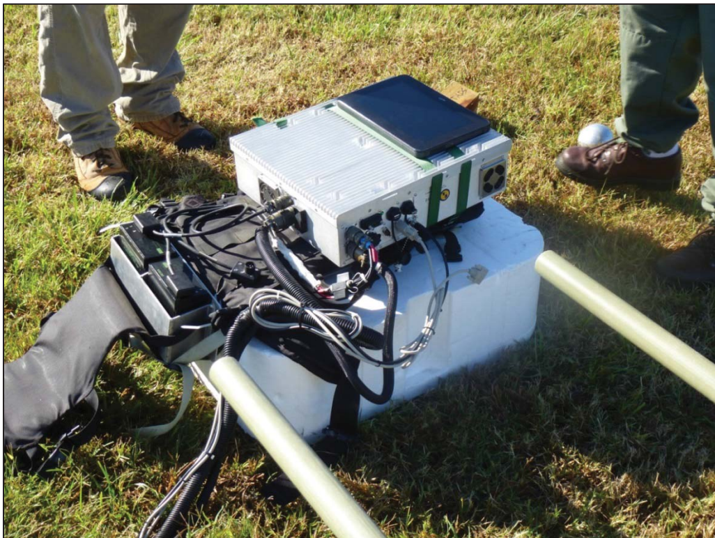
Figure 2. TEMTADS Computer Mounted on Original Backpack (Open for Inspection)
