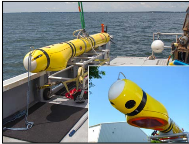
Figure 4. The REMUS 600 AUV on deck ready for deployment. The bulge in the forward wet section was to accommodate for the dual echosounder transducers (inset). The section aft houses the electronics for data acquisition and processing.
