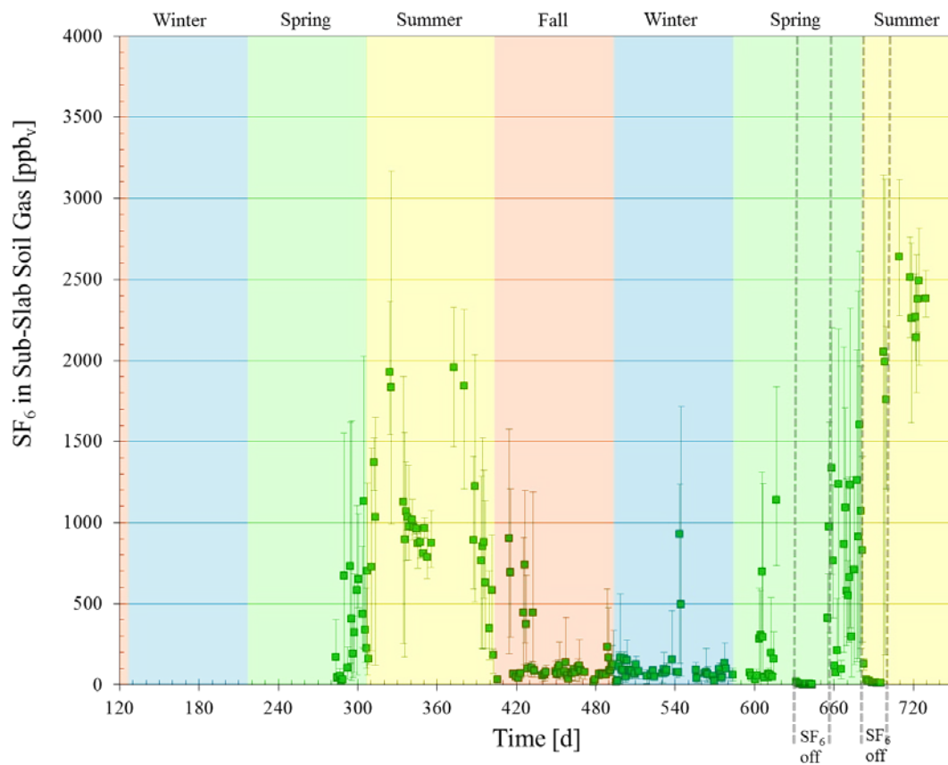
Figure A.25. 24-h averaged \text{SF}_6 concentrations sub-slab soil gas at location 5 from winter 2010 through summer 2012 with error bars spanning the daily maximum and minimum values.
