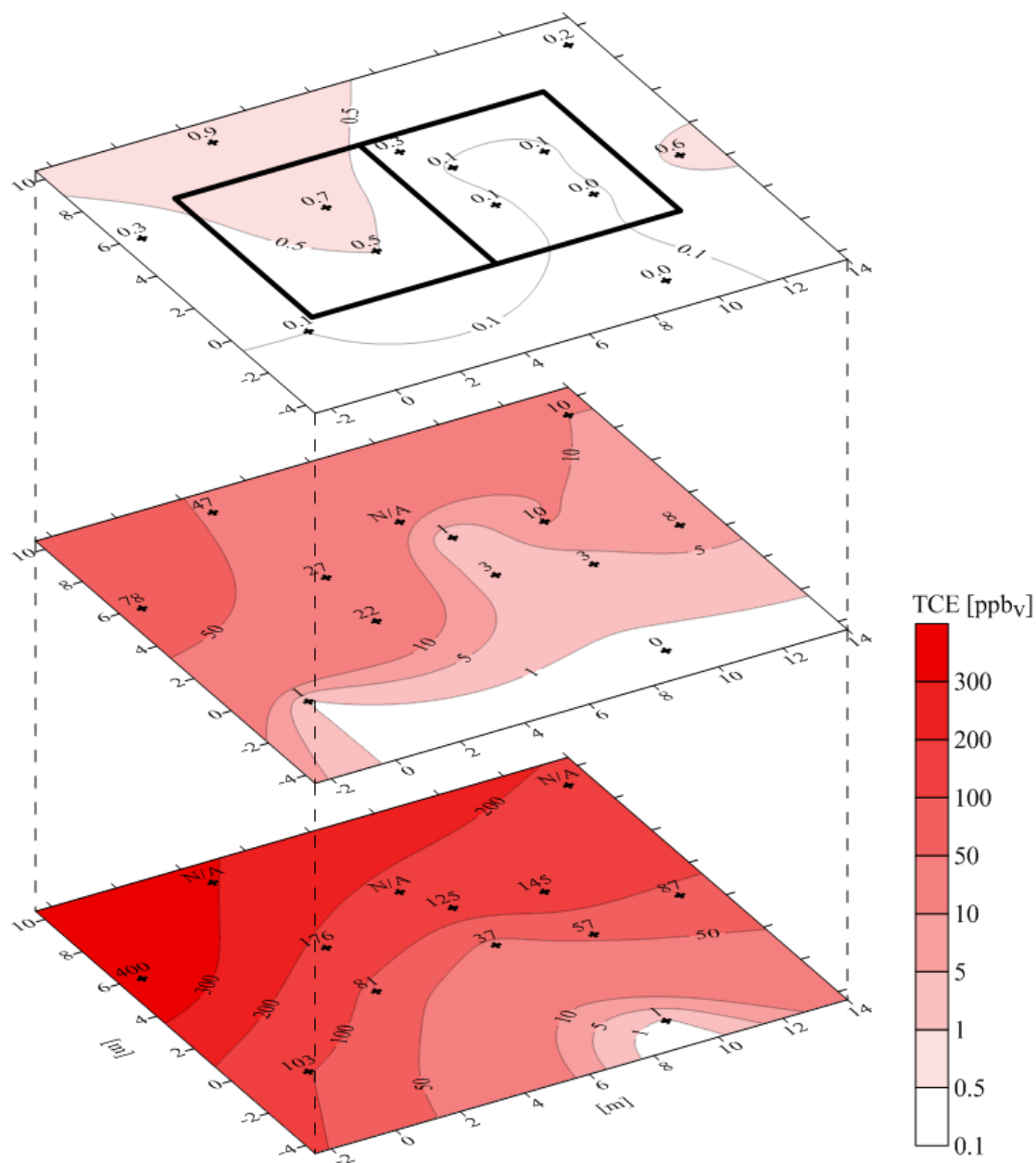
Figure A.11. Multi-depth contour plot of TCE in soil gas for samples collected and analyzed from September 29 th to September 30 th , 2011.
