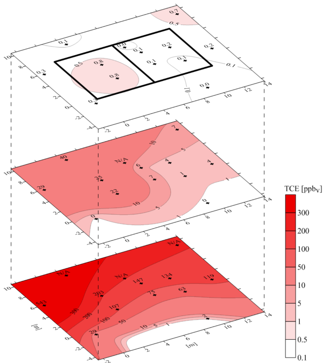
Figure A.4. Multi-depth contour plot of TCE in soil gas for samples collected and analyzed from November 13 th to November 15 th , 2010.
