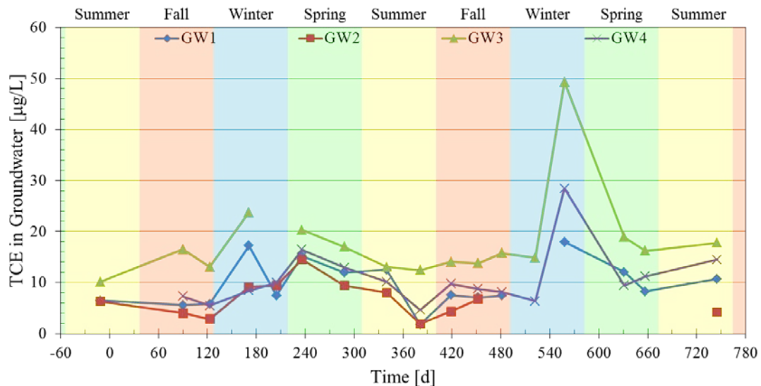
Figure 4.10. TCE groundwater concentrations at shallow exterior sampling points from August 2010 to August 2012.
