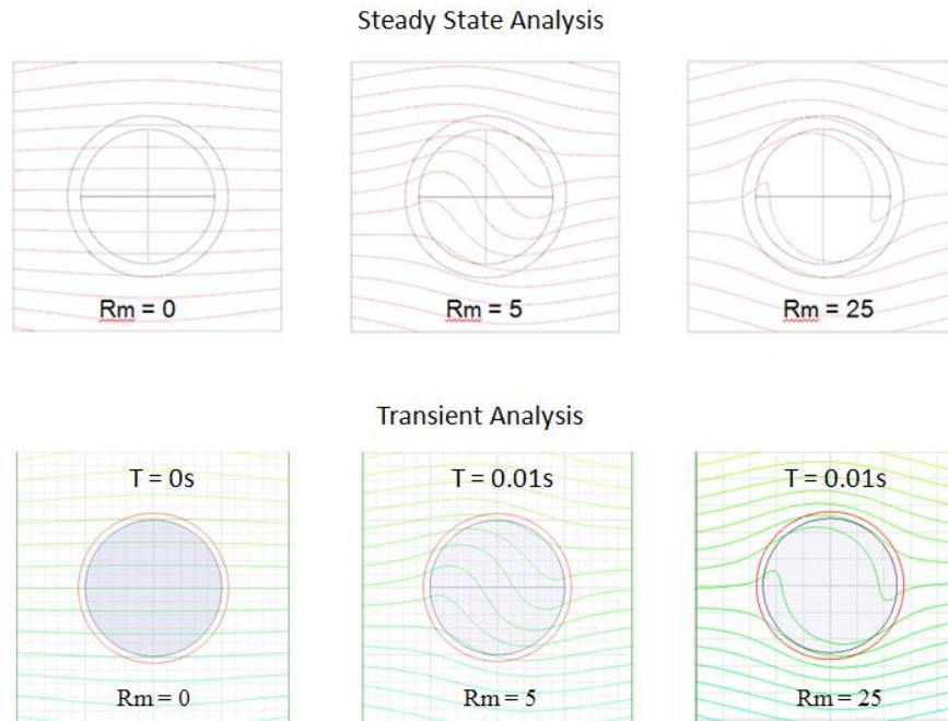
Figure 2 Resulting magnetic flux lines for the cylinder of relative permeability 1.0
