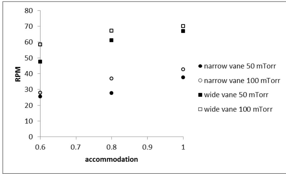
Figure 16. Angular Speed with Varied Accommodation (Simulation)
