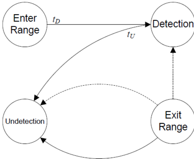
Figure 12. Mediator event graph
