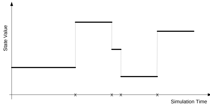
Figure 6. DES state trajectory
