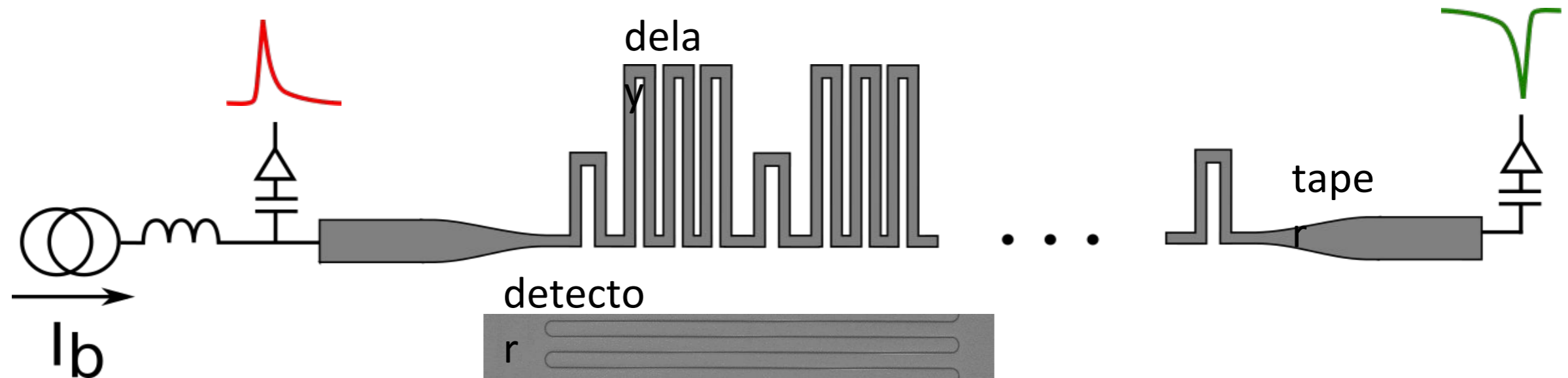
Microstrip line
