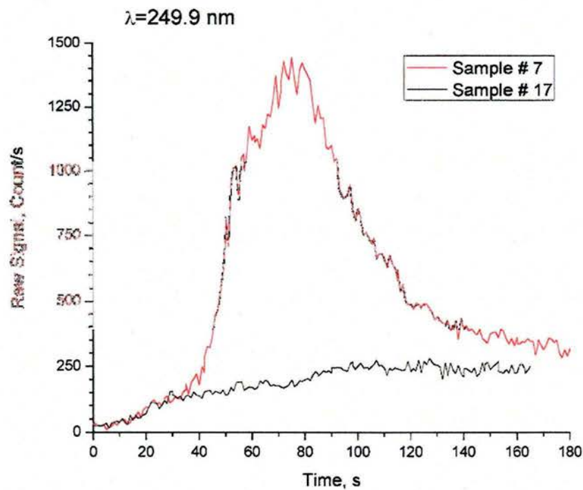
Figure 10 : Temporal evolution of the measured raw signal at 249.9 nm
